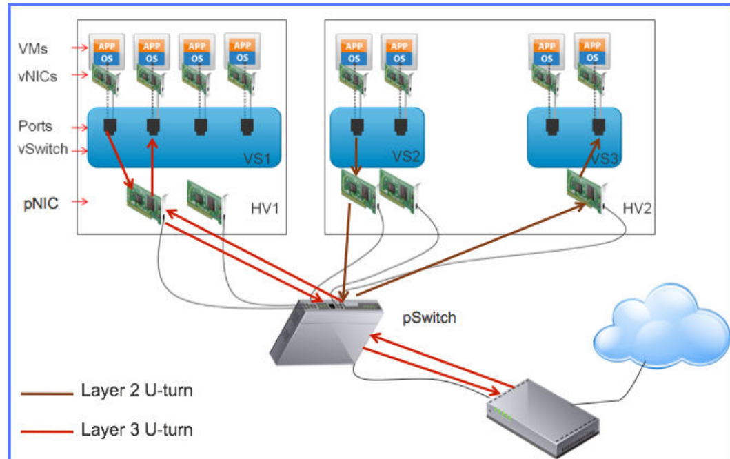
Figure 2-18. Hair-pinning Traffic
