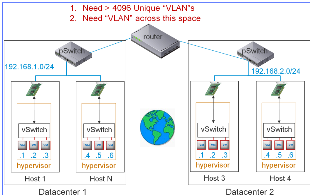
Figure 2-22. Problems solved by VxLAN, with Sample Network
