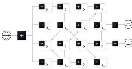
Figure 5: A theoretical dynamic network topology with each service fronted by load balancers.
