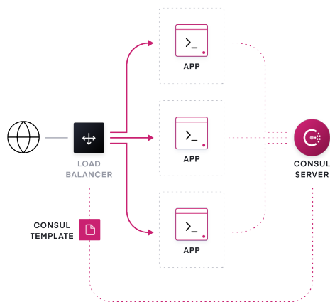
Figure 9: A dynamic network topology with HashiCorp Consul handling east-west traffic and service-to-service communication, while a load balancer balances north-south traffic.
