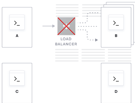
Figure 6: Despite service B's redundancy, if the only load balancer goes down, all instances of service B are unavailable.
