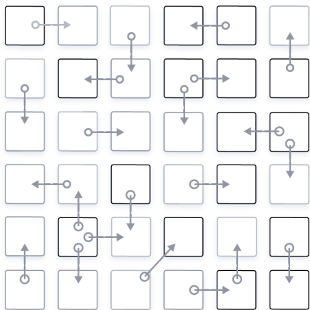
Figure 4: Communication patterns in a simple microservices application.
