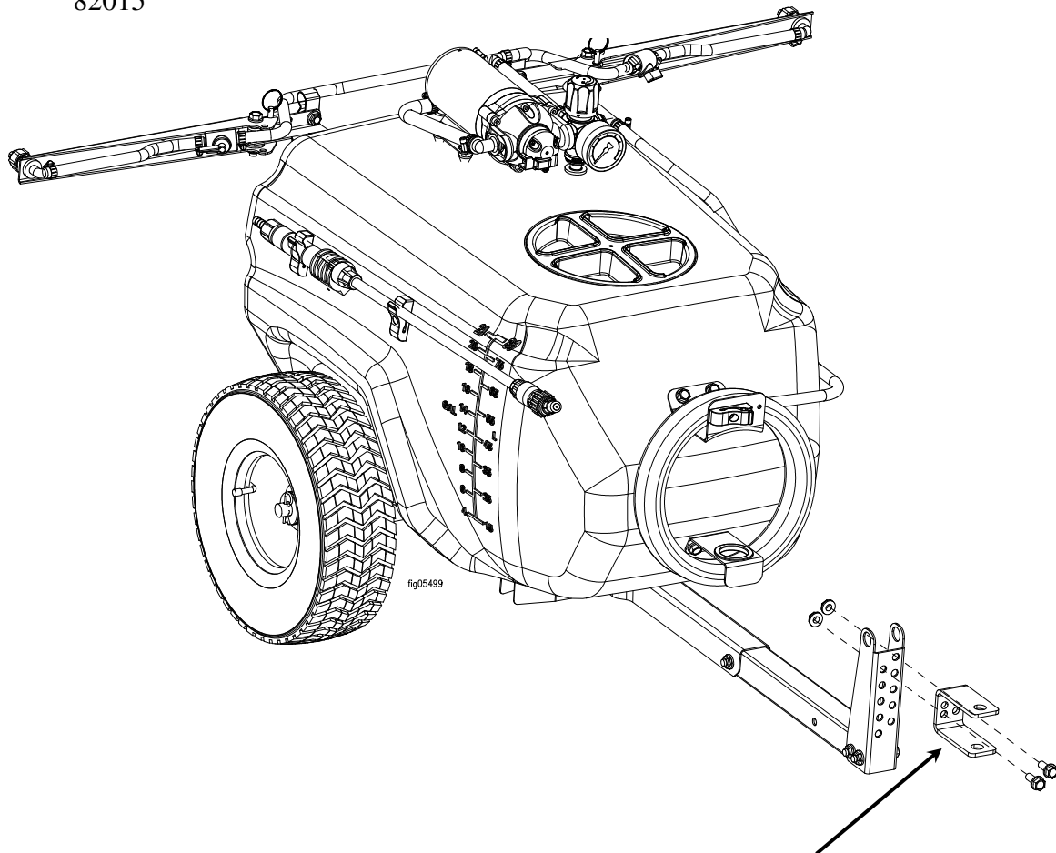
Hitch bracket
