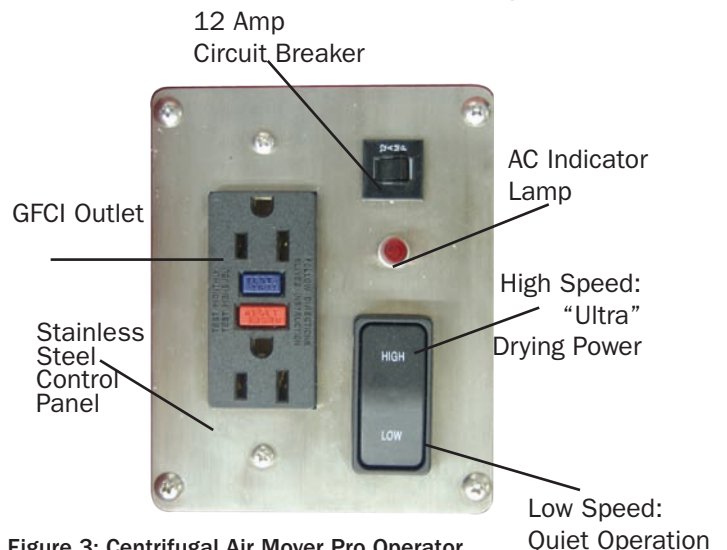
Figure 3: Centrifugal Air Mover Pro Operator Panel
