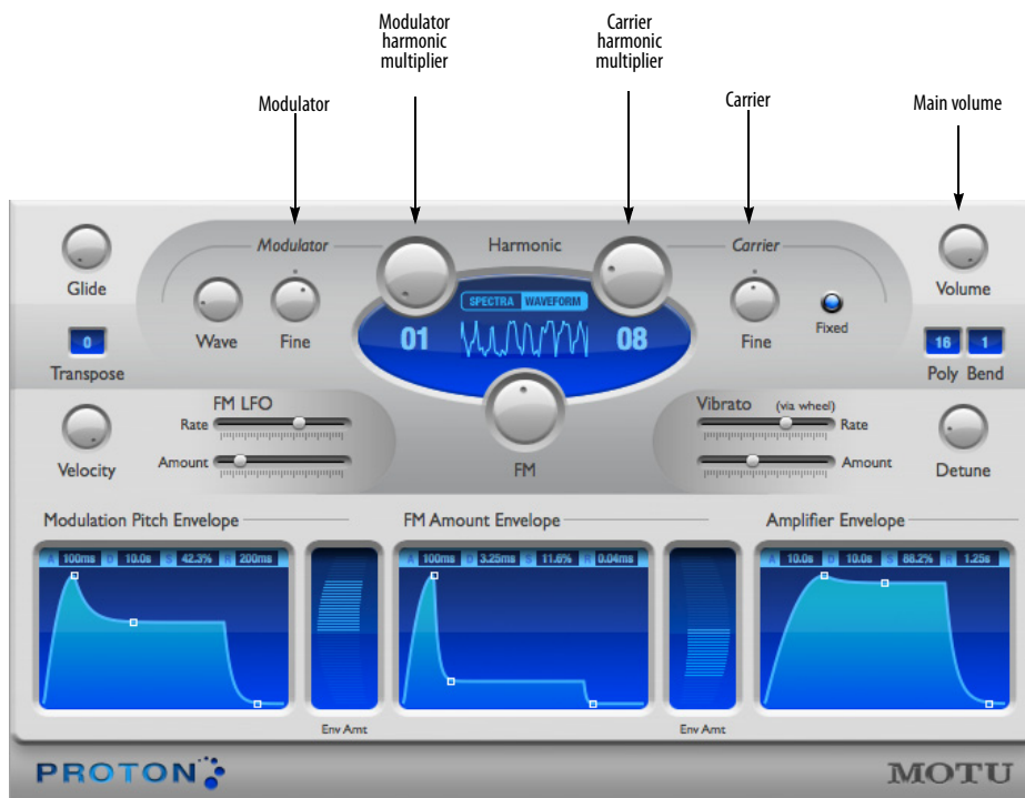
Figure 2-30: Proton.
