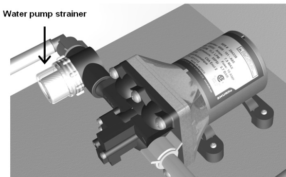
Water pump
