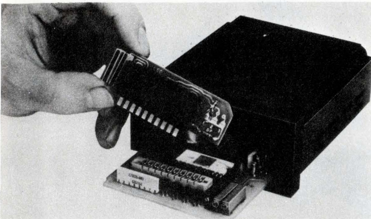
Weston's 1295 is one of the few low-cost DPMs to offer an LED display. The meter also incorporates a custom LSI chip from Mostek in the digital portion.
