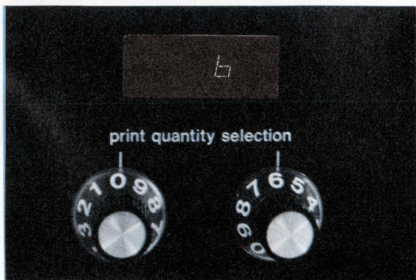
Convergence. This detail of the electromechanical counter of a Xerox 1000 copier shows the static backlit numbers. When the left-hand number, representing copies produced, reaches parity (coincides) with the right hand number, representing copies requested, the copying mode automatically shuts off.
