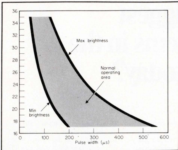
Display pulse width vs voltage. The Hoffman display subsystem typically operates at 27 V and 175 \mu s pulse width every 6,400 \mu s.
