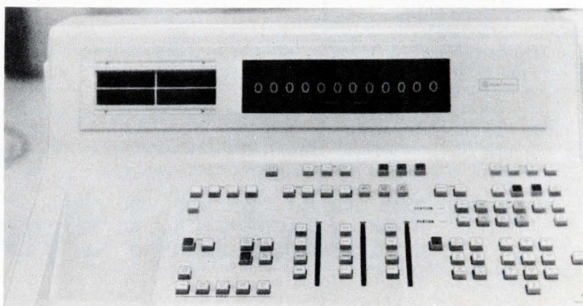
The Traffic Service Position Switchboard with 12-digit Nixie display. There are over 5000 of these units now in service throughout the country. Presently in the development stage, a new version of the switchboard will use seven-segment LED displays.
