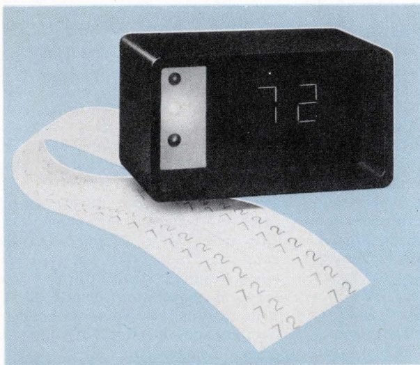
This Rotiform display unit is used in digital speedometers, and to display transducer outputs in shipboard applications.
