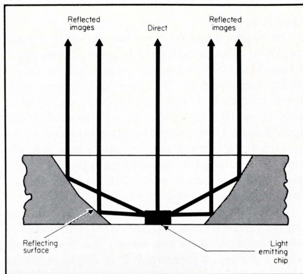
This LED display , the SLA-1 from Opcoa, reflects the multi-directional light output from GaP to reduce the actual amount of semiconductor material in the display. Displays that do not use this technique can require up to 10 times as much semiconductor material.
