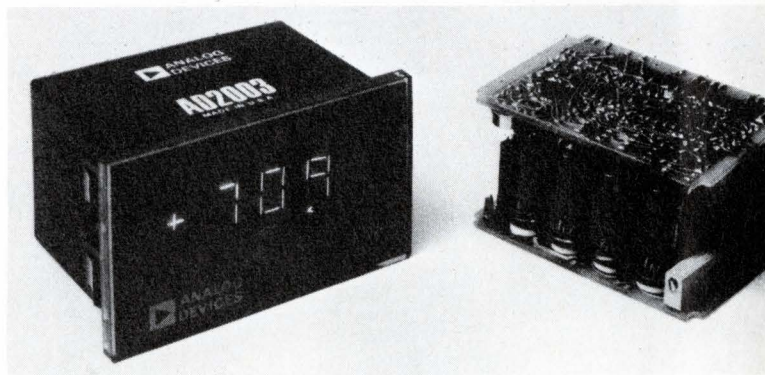
The latest, low-cost DPM from Analog Devices is the AD2003. The meter is aimed specifically at high performance applications such as instrumentation and data collection, and includes such features as a true differential input and latched BCD outputs.
