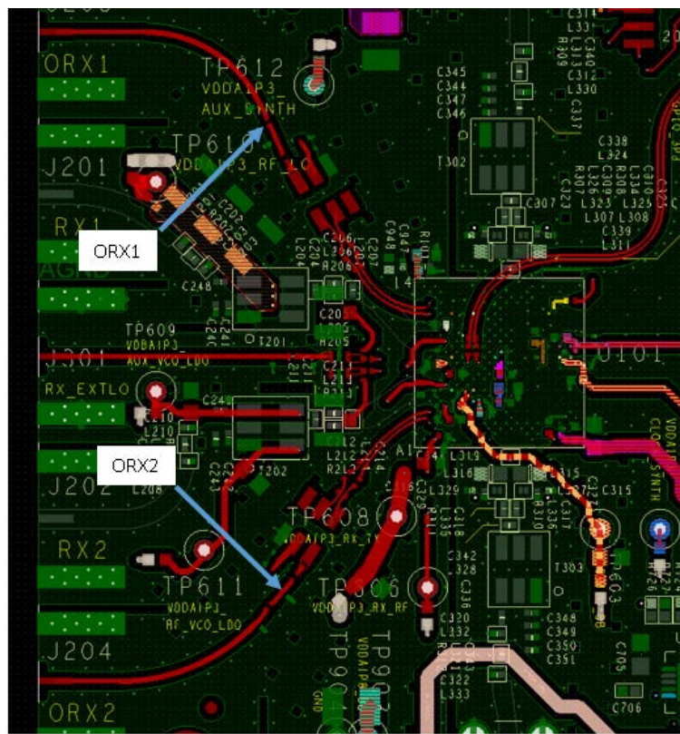
Figure 278. Pi Network Matching Components Available on Observation Receiver Inputs
