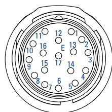
Resolver Connector
