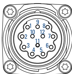
Resolver Connector
