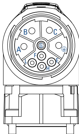
Power Connector
