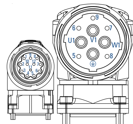
Resolver Connector
