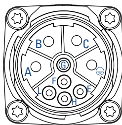
Power Connector
