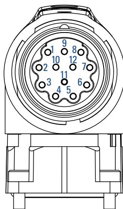
Resolver Connector
