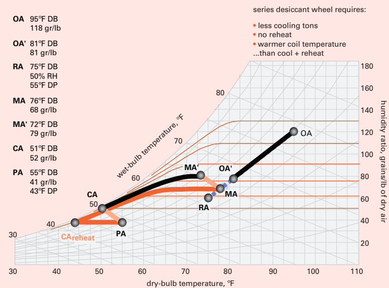
Figure 14. Performance of dual-wheel primary AHU
