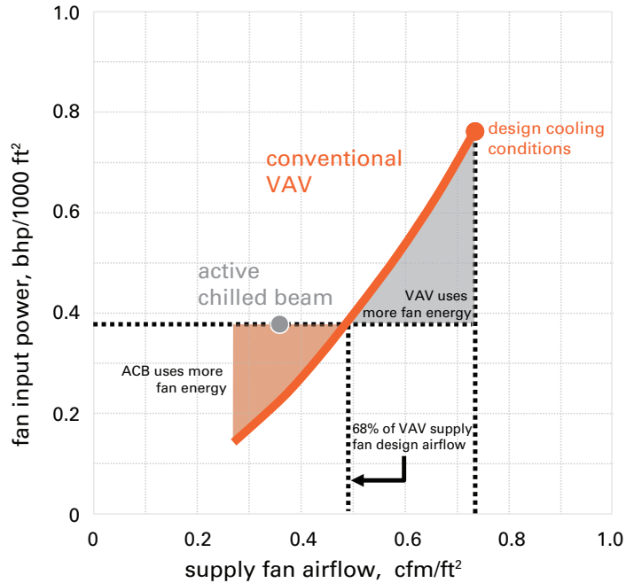
Figure 6. Supply fan power at part load (ACB vs. conventional VAV)
