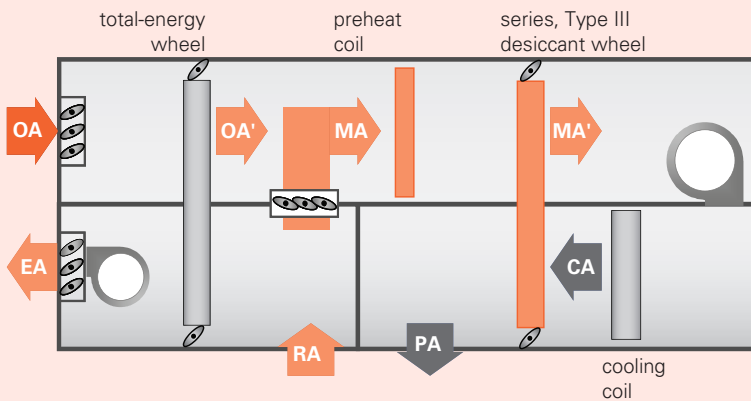
Figure 13. Example primary air-handling unit for an active chilled beam system
