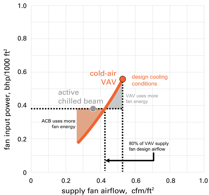
Figure 7. Supply fan power at part load (ACB vs. cold-air VAV)
