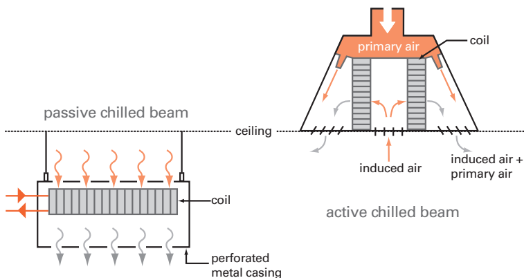
Figure 1. Passive versus active chilled beams
