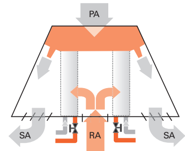
Figure 3. Primary airflow (PA) in an active chilled beam.
