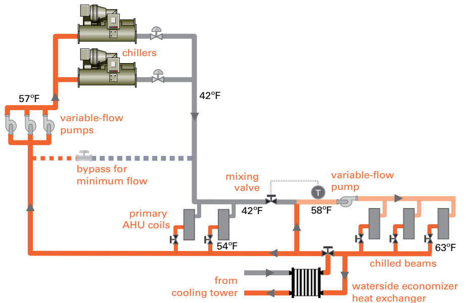
Figure 8. Shared chilled-water plant with waterside economizer
