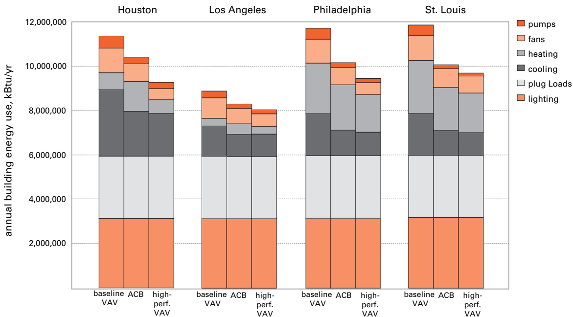
Figure 10. Comparison of annual energy use for an example office building
