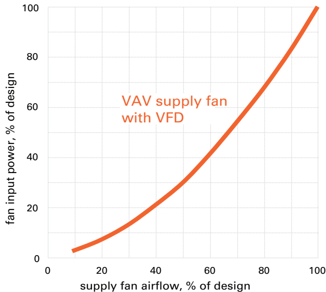
Figure 5. Part-load performance of a typical VAV system supply fan
