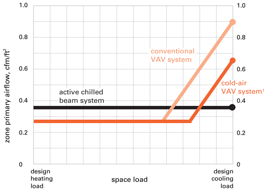
Figure 4. Zone primary airflow at part load
