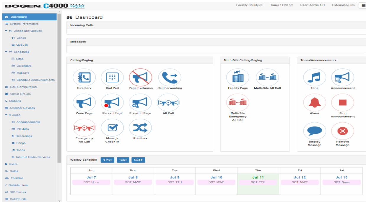
Figure 1-5, C4000 Dashboard
