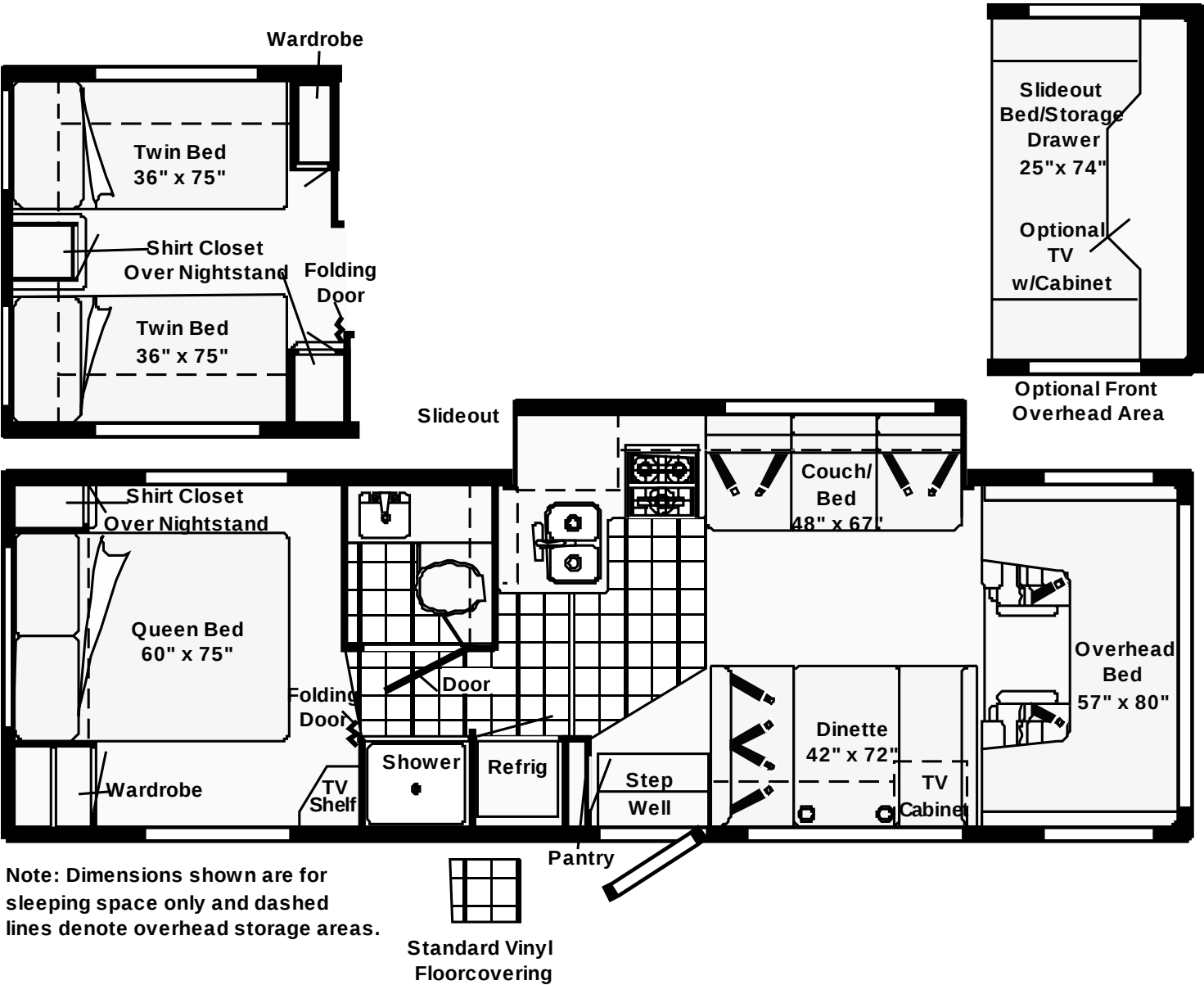
FLOORPLAN
