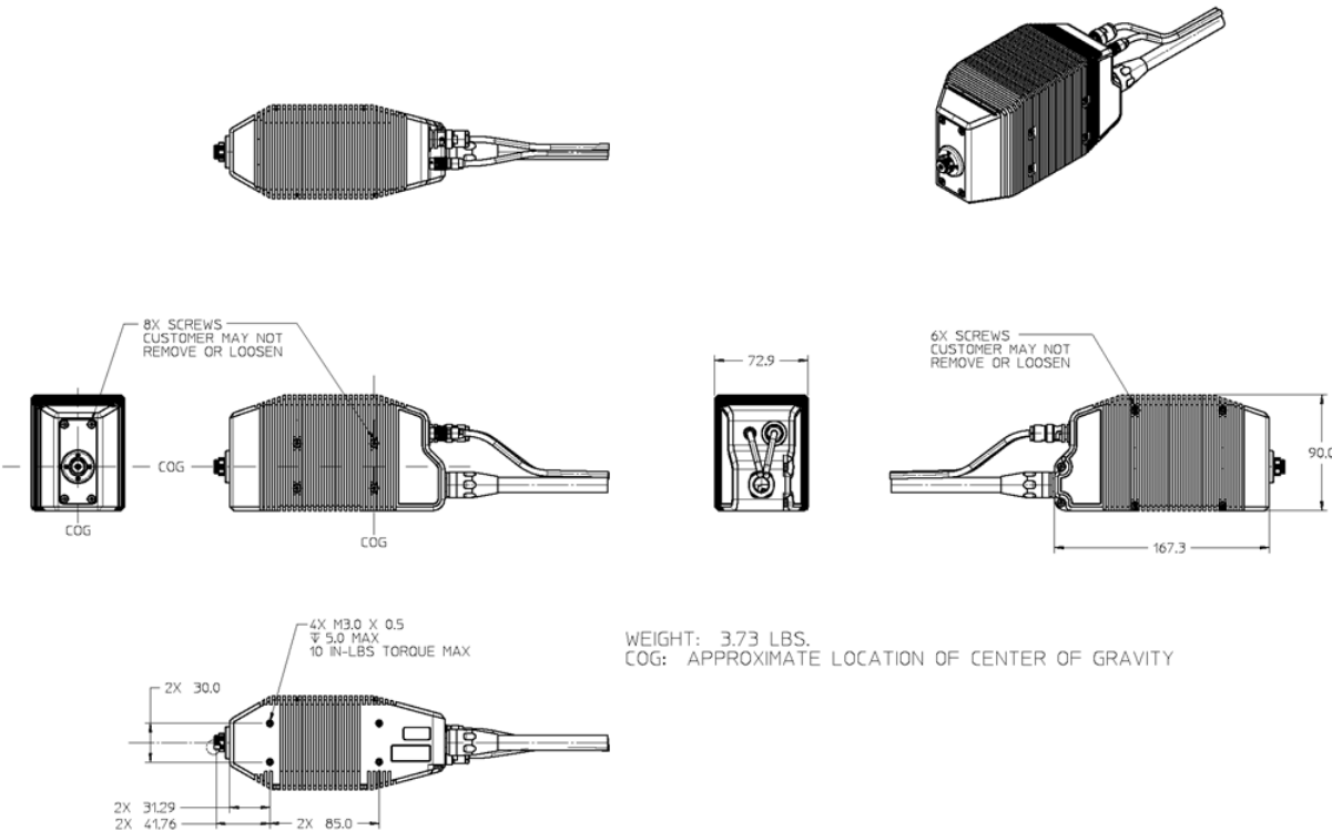
Figure 2-10 N5293/5AX03 Millimeter-wave module Mechanical Specifications
