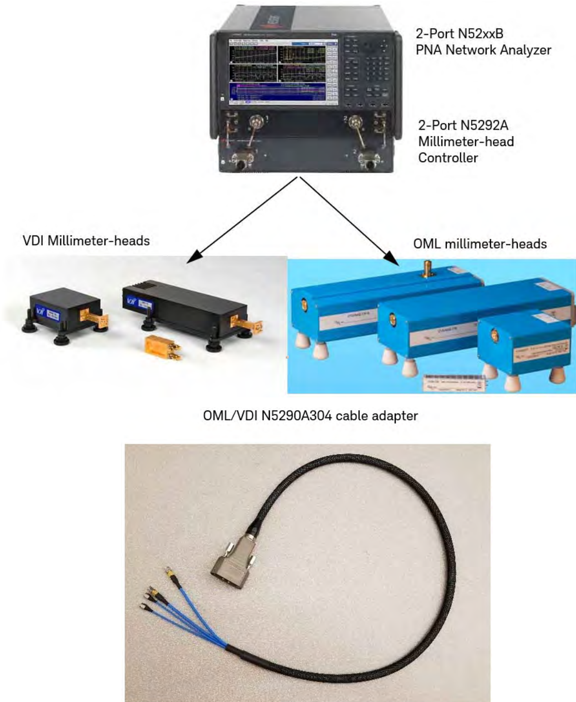
Figure 2-3 N52xxB 2-Port Banded Test System – Coaxial Measurement Configuration (using OML/VDI Millimeter Heads)
