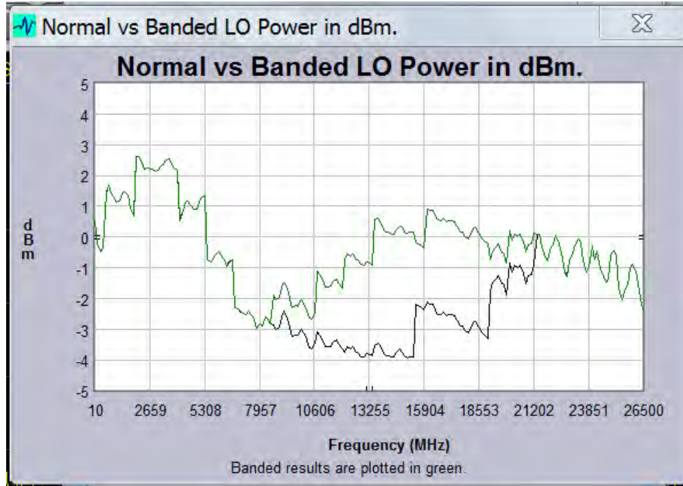
Figure 3-19 Normal vs. Banded LO Banded Power in dBm
