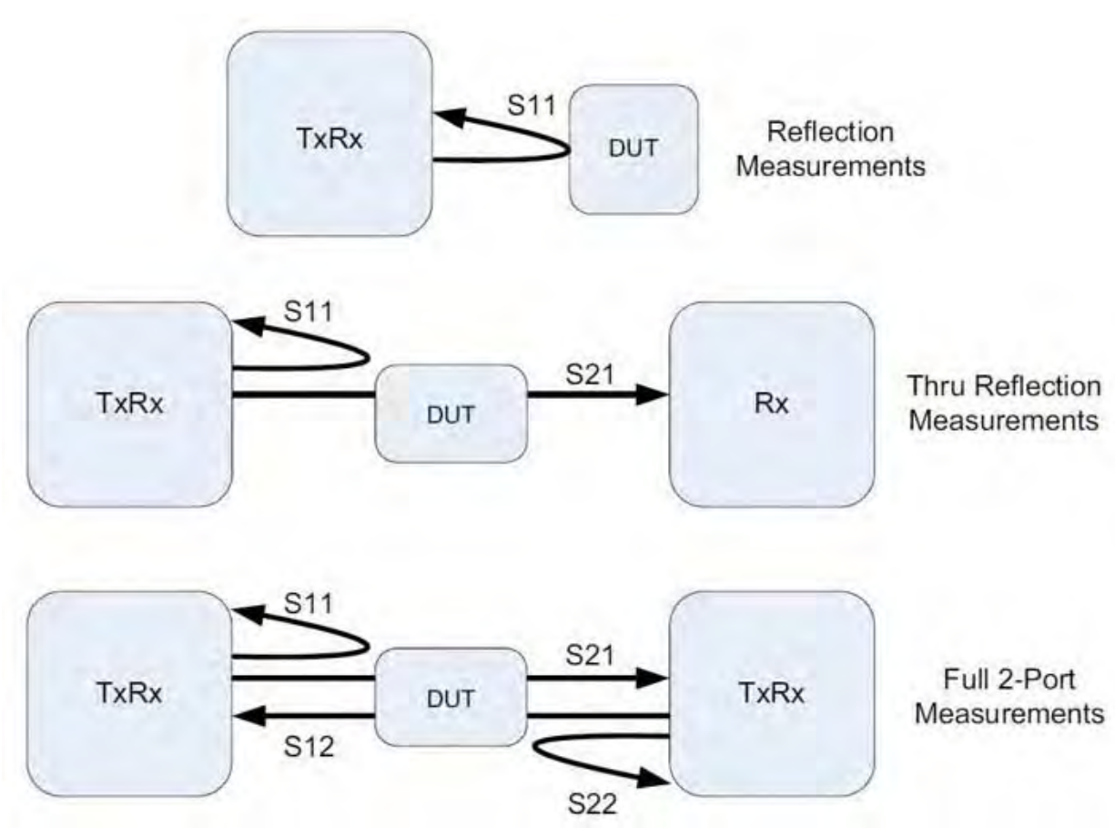
Figure 2-11 Module Configurations
