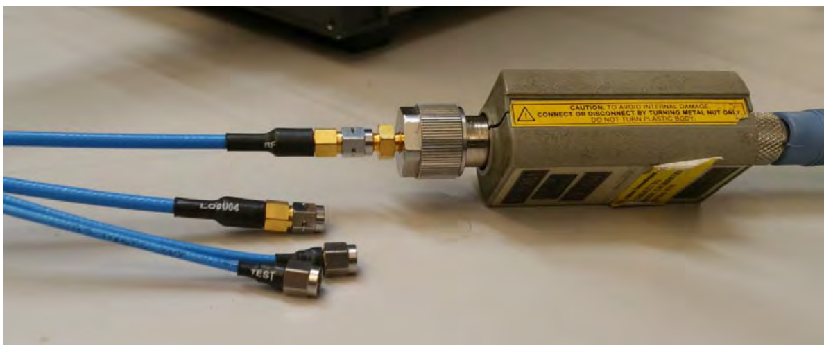
Figure 3-21 Connect the Power Meter to N5290A304 Adapter Cable
