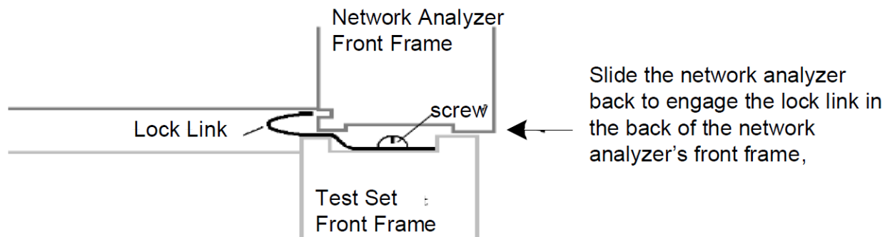
Figure 3-5 Locking the Analyzer using the vertical links
