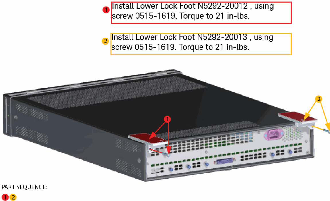
Figure 3-4 Install lower lock feet N5292-20012 and N5292-20013 using screws 0515-1619.
