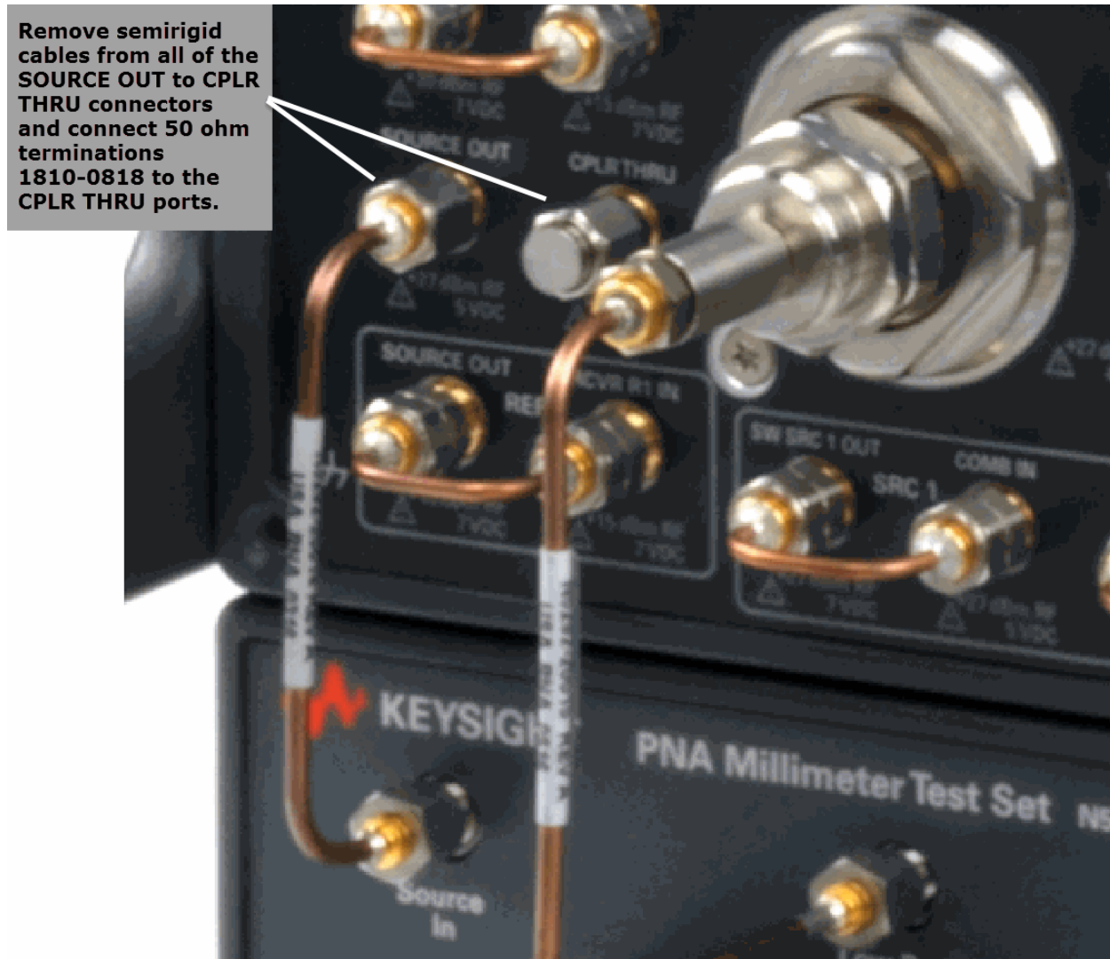
Figure 3-7 Remove Semirigid Cables and Connect 50 termination (1810-0118) to the CPLR THRU Ports
