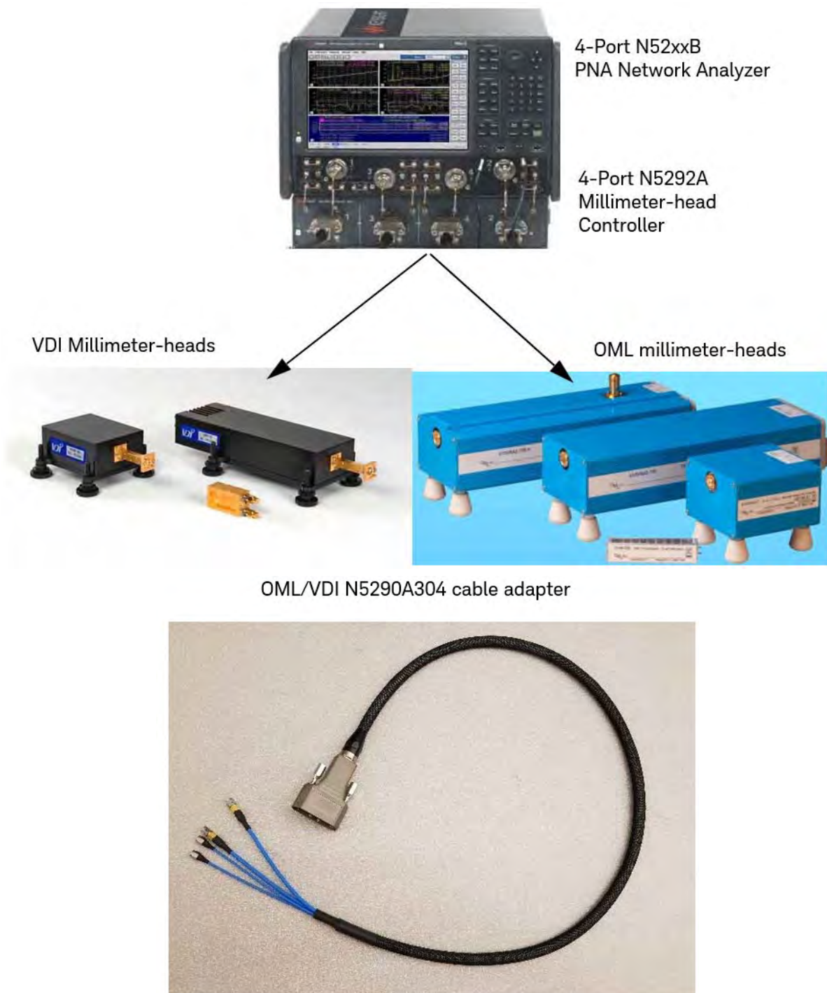
Figure 2-4 N52xxB 4-Port Banded Test System – Coaxial Measurement Configuration (using OML/VDI Millimeter Heads)
