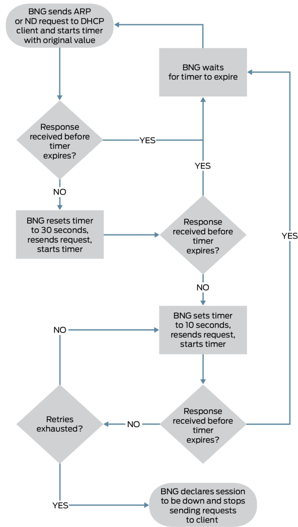
Figure 15: Layer 2 Liveness Detection Send Behavior Flow
