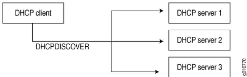
Figure 3: DHCP Discover
