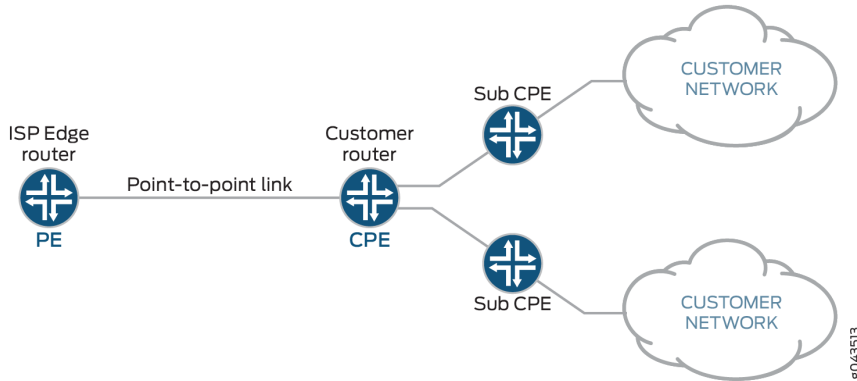
Figure 9: Sub-prefix Delegation
