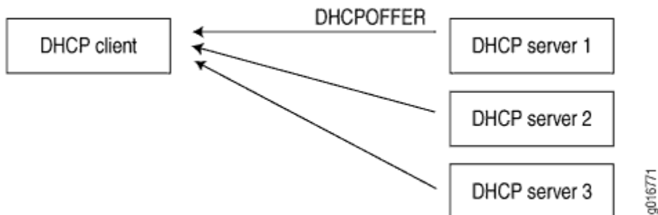
Figure 4: DHCP Offer
