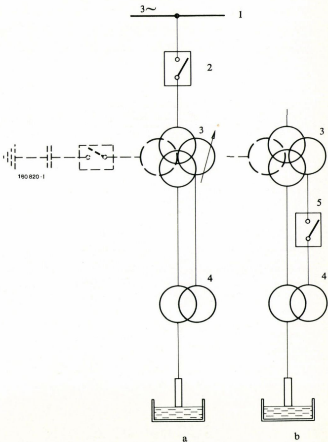
Fig. 9 – Power supply to an arc furnace through a main transformer with three windings (possibly also with a fourth winding for connection to a capacitor bank for improving p.f.) and a series transformer
