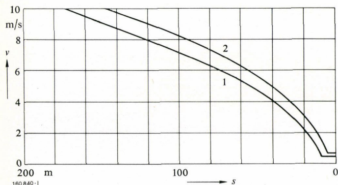
Fig. 6 – Approach curves
