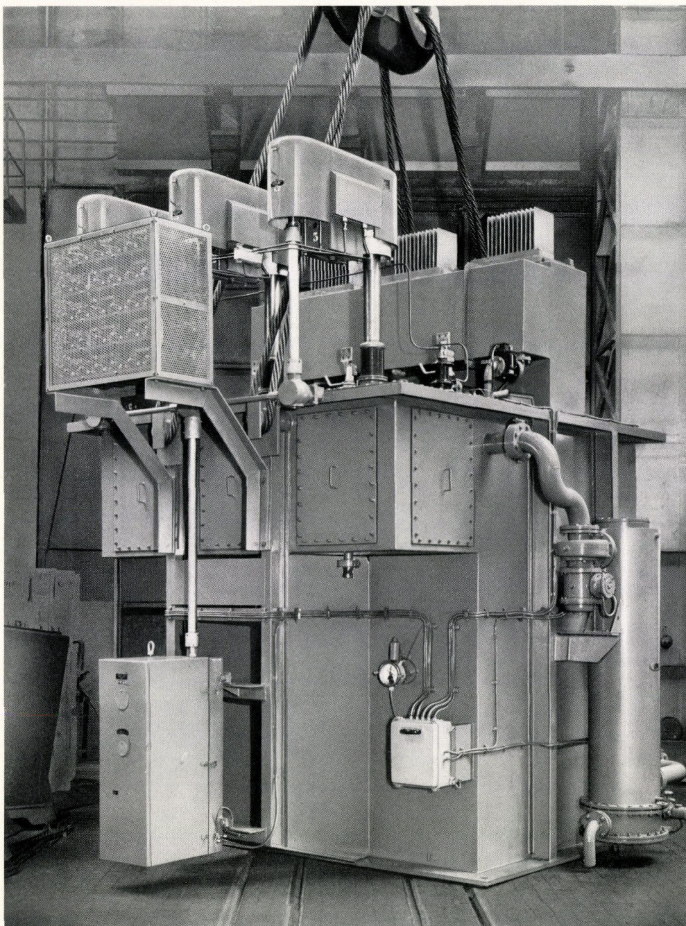
Fig. 5 – Three-phase furnace transformer for indoor installation, with circulating oil and water cooling
