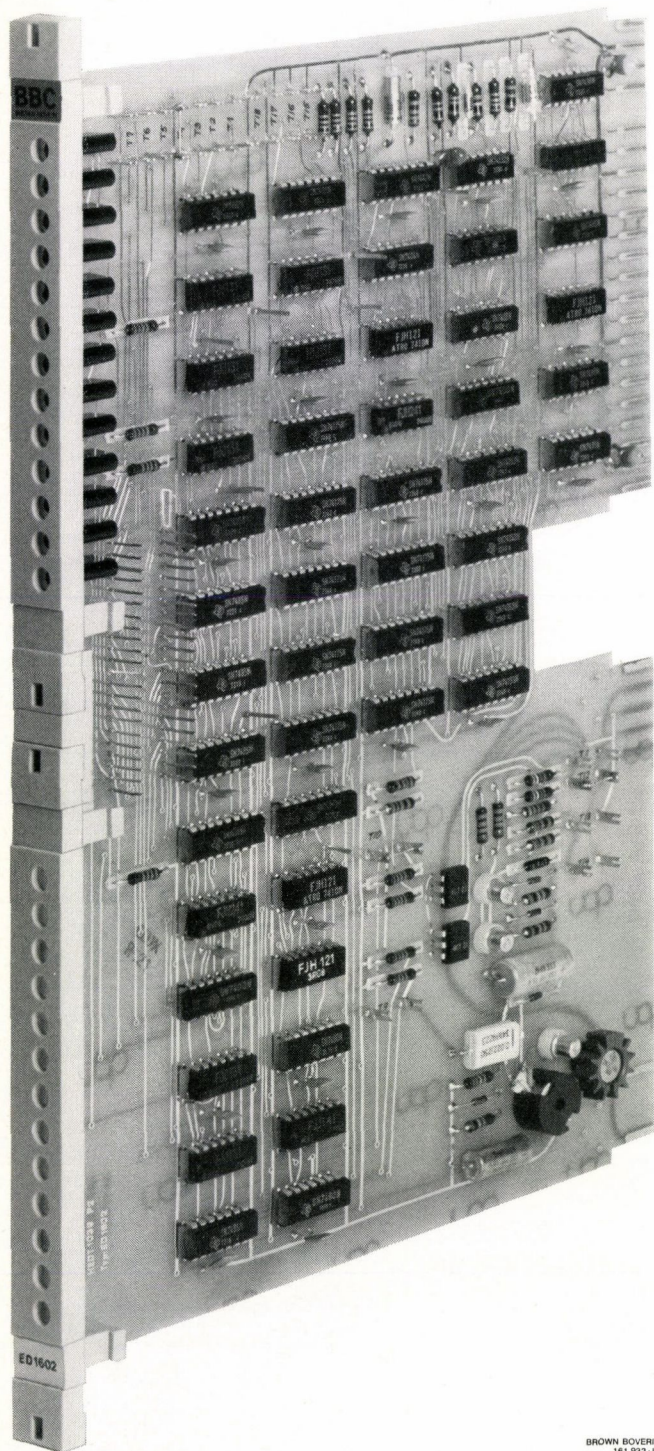
Fig. 3 – Peripheral unit module
