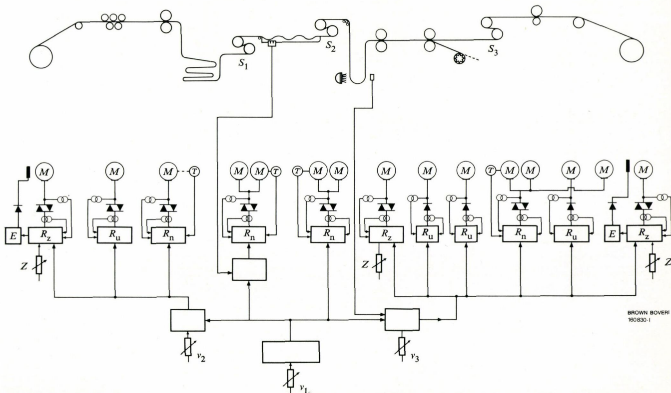
Fig. 2 - Strip flow diagram for the pickling line
