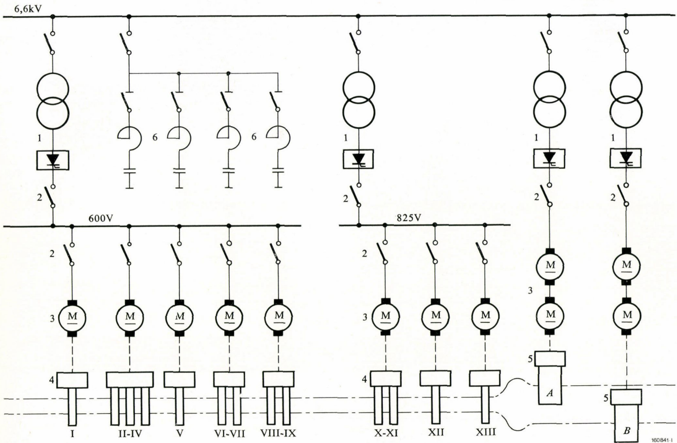
Fig. 1 - Combined electrical and mechanical arrangement of main drives and their supply
