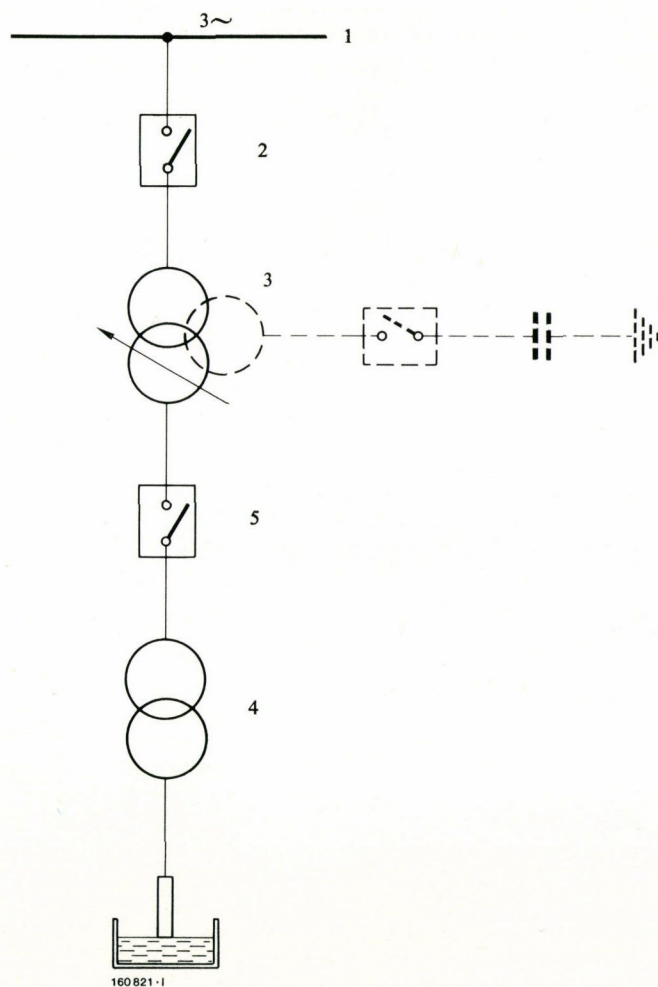
Fig. 11 – Power supply for a high-capacity arc furnace through a regulating transformer and a unit-connected, fixed-ratio furnace transformer
