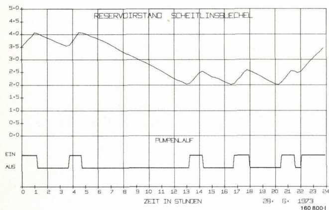
Fig. 5 – Example of a plotter diagram. The bottom half of the diagram shows the running times throughout a day of a pump filling the reservoir indicated in the upper part of the diagram, together with its level.
