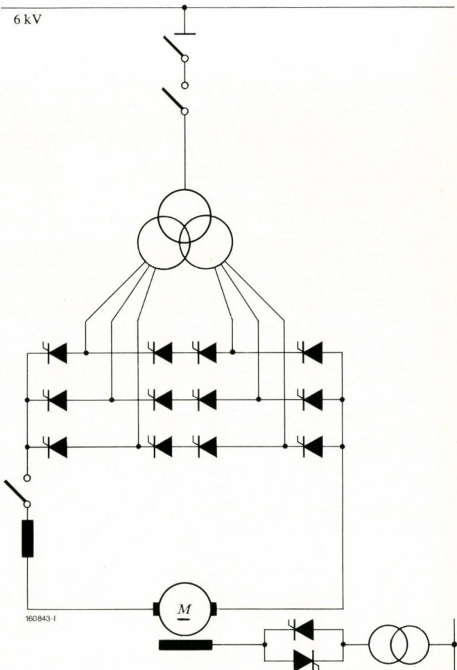
Fig. 1 – Circuit of thyristor supply equipment
