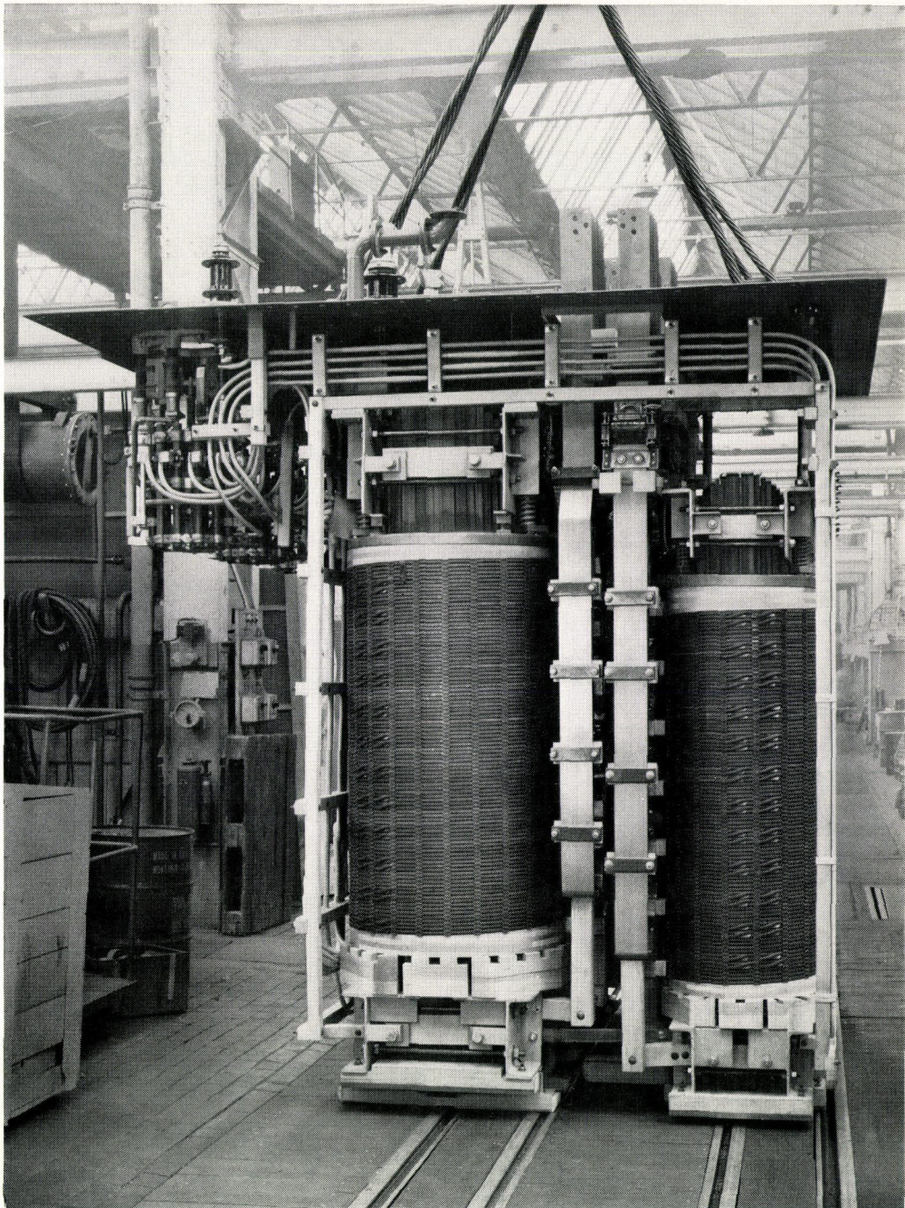
Fig. 6 – Internals of the transformer shown in Fig. 5
