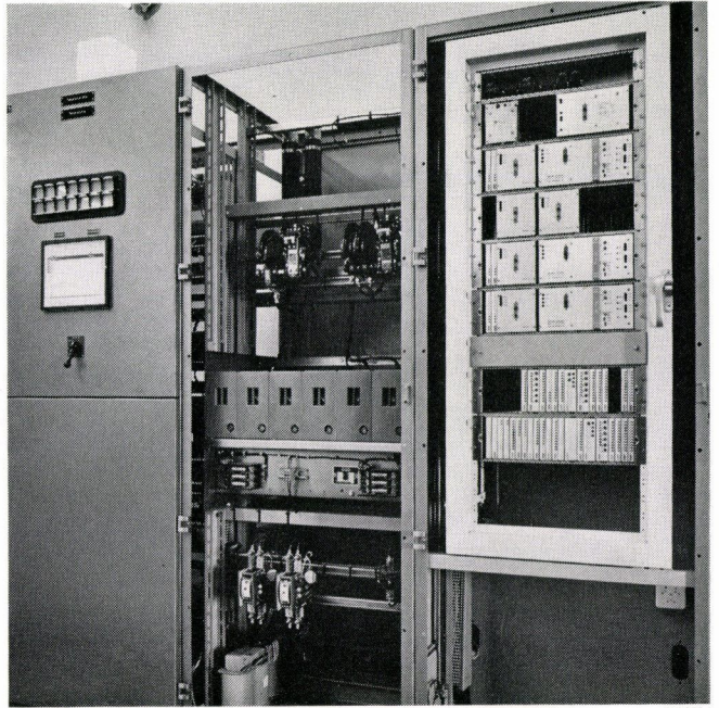
Fig. 3 – Switchgear cabinets with front panels removed
