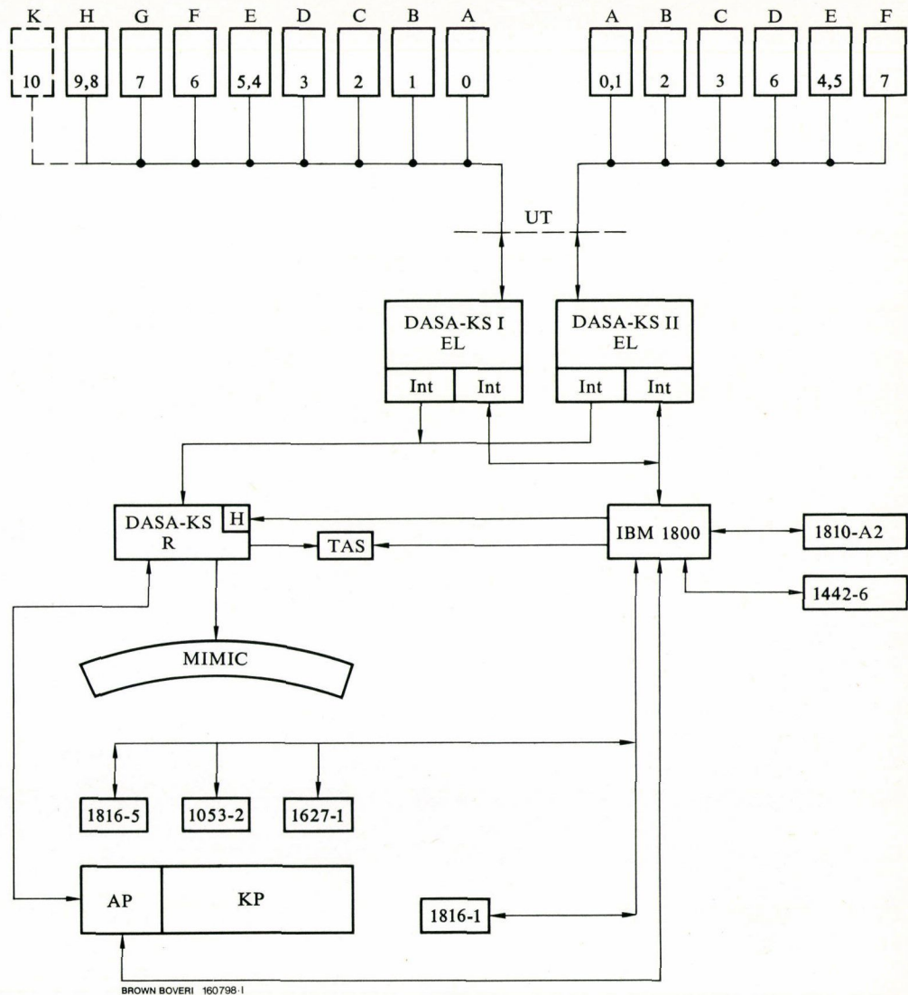
Fig. 4 – Block diagram of the complete control system
