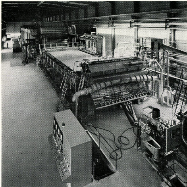
Fig. 1 – Paper machine and controls
