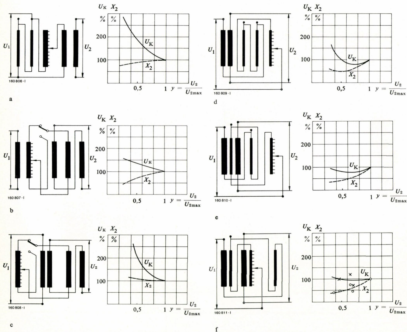
Fig. 4 – Variation of short-circuit voltage U_K and reactance X_2 , referred to secondary side, of furnace transformers in various configurations (a to f) as a function of factor y = \frac{U_2}{U_{2max}}
