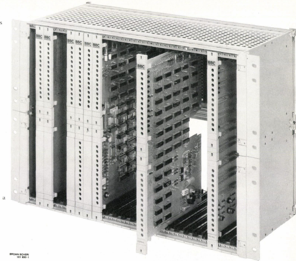
Fig. 2 – Tier arrangement a: Front view b: Rear view showing system bus
