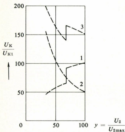
Fig. 14 – Variation of impedance voltage U_K of transformer group in Fig. 11 with winding configuration different from those in Fig. 12 and 13
