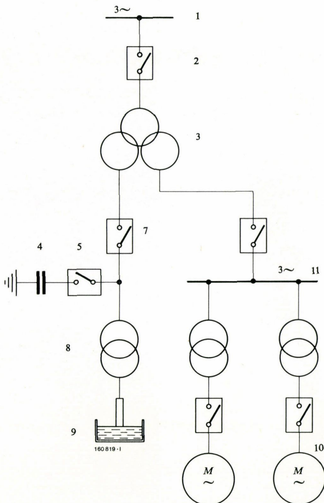
Fig. 8 – Power supply to a high-capacity arc furnace through a furnace transformer with three windings so as not to influence other loads
