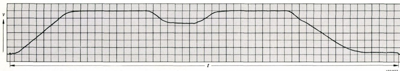
Fig. 2 - Speed/time diagram of Signalbahn, St. Moritz
