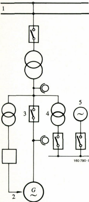
Fig. 1 - Plant with generator breaker 1 = E.H.V. network 2 = Rectifier excitation 3 = Generator breaker 4 = Auxiliary transformer 5 = Standby diesel generator set
