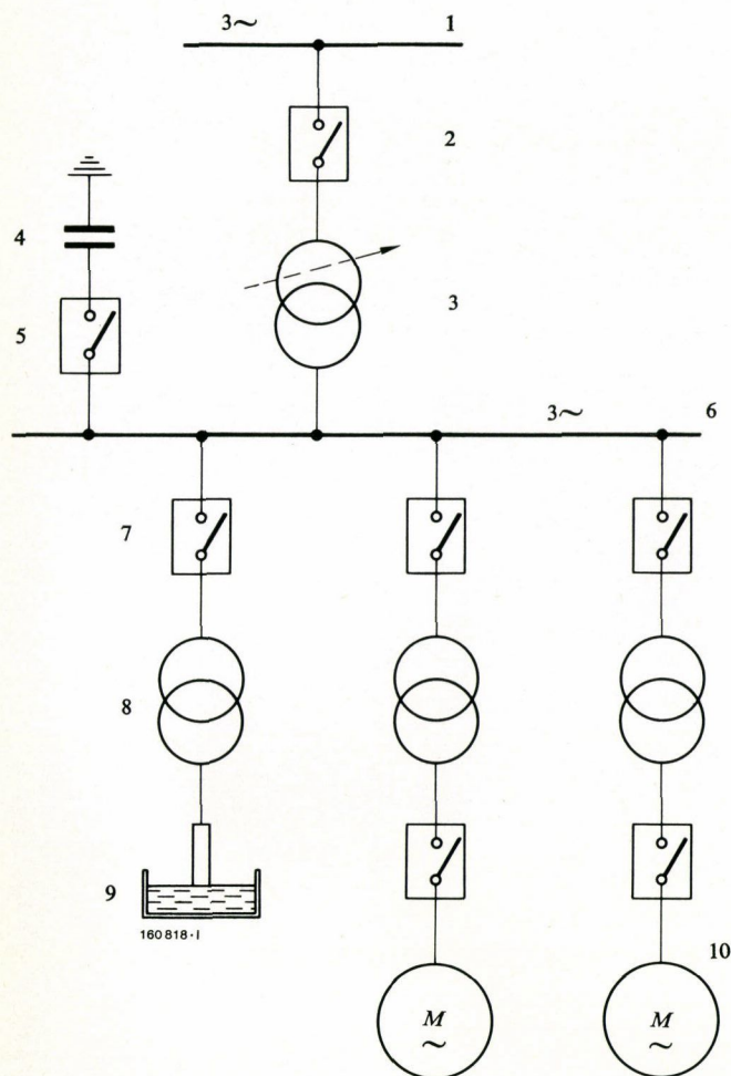
Fig. 7 – Diagram of power supply to a steelworks with an arc furnace installation, the power of which is negligible compared with the total installed power
