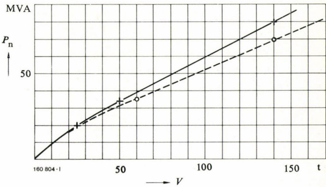
Fig. 2 – Nominal rating P_n of furnace transformers as a function of furnace capacity V (tonnes)
