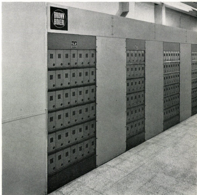
Fig. 6 – Thyristors for supplying main d.c. drives
