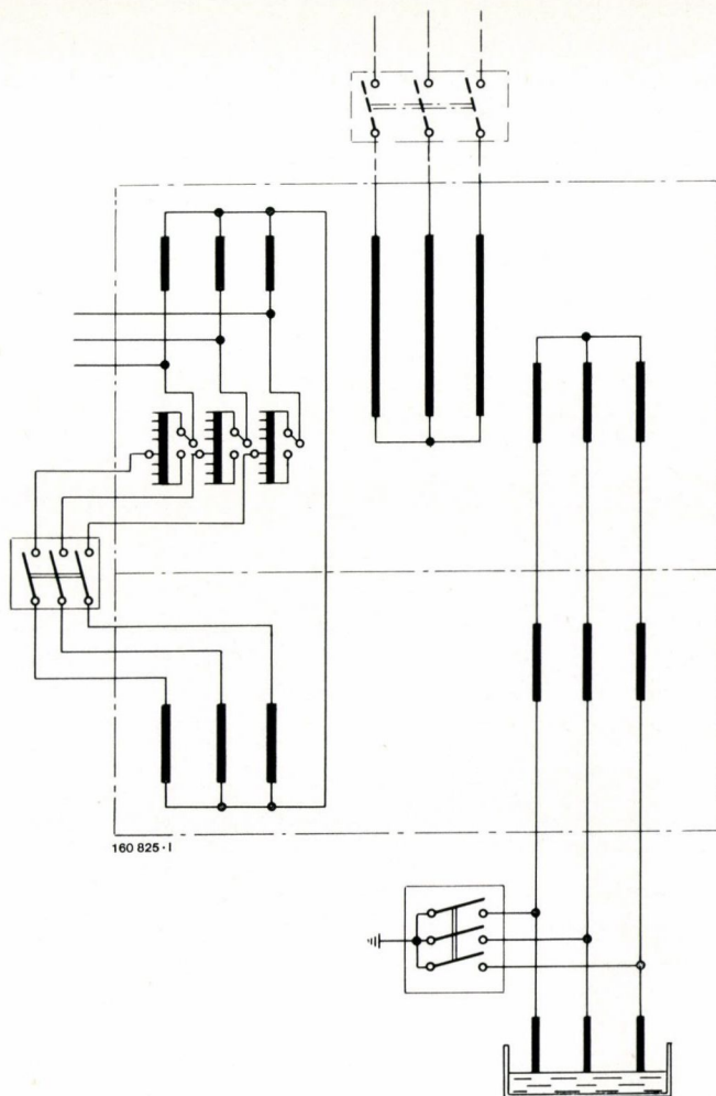
Fig. 15 – Winding arrangement of transformer group with breaker in intermediate circuit as in Fig. 9 b
