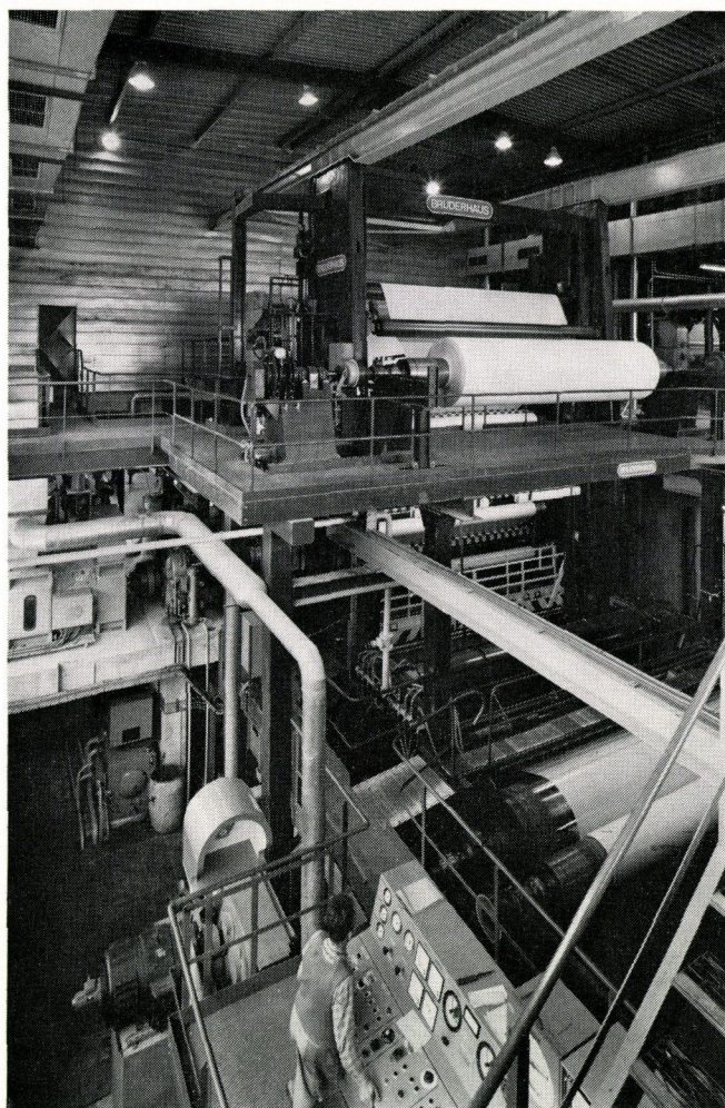
Fig. 3 – Supercalender with reelers, main drive and controls
