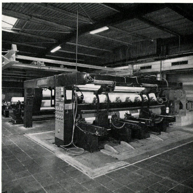
Fig. 4 – Slitter-rewinder with controls built into machine frame
