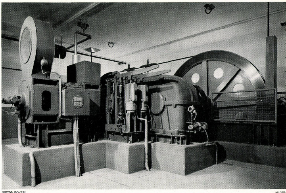
Fig. 1 – Machine room of Signalbahn, St. Moritz
