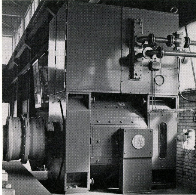
Fig. 2 – 1725 kW d.c. drive motor with built-on heat exchanger
