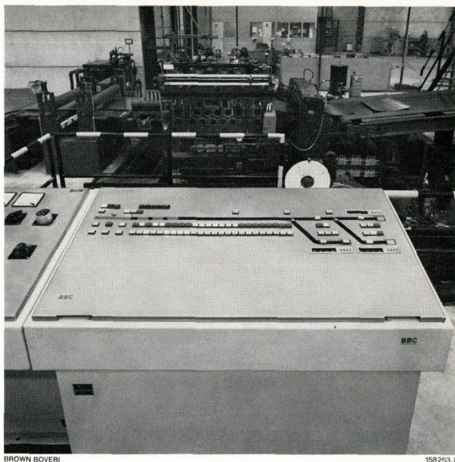
Fig. 8 – Main control desk for cut-to-length line
