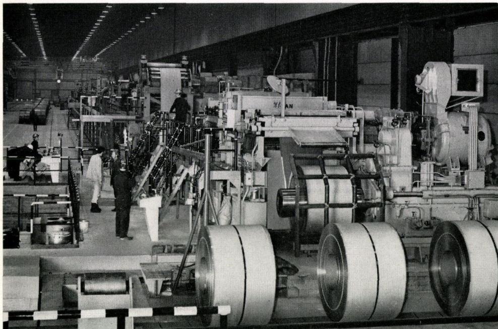
Fig. 4 – Coil changing (exit section) at the pickling line
