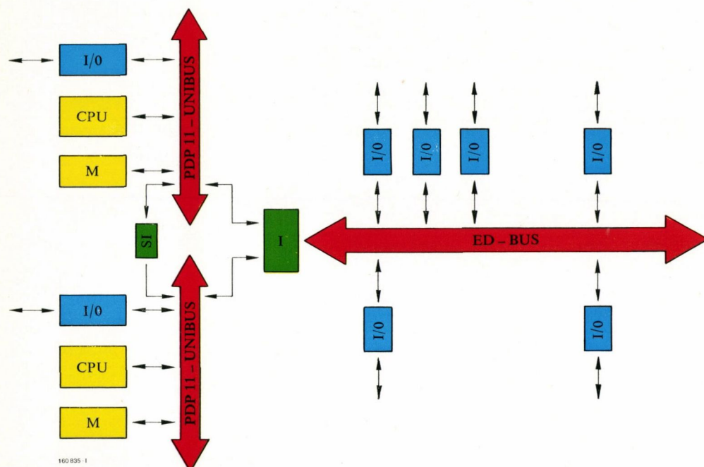
Fig. 5 – Dual computer systems
