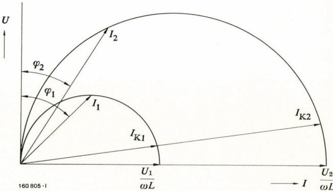
Fig. 3 – Circle diagram of an arc furnace (for symbols see text)
