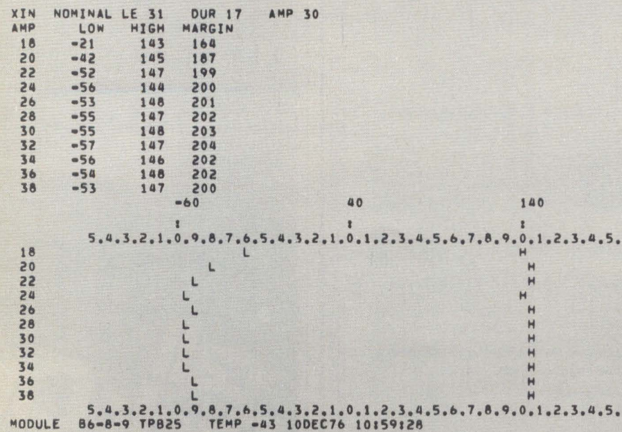
◀ Fig 8e Similar to (8d) for the transfer in function.
