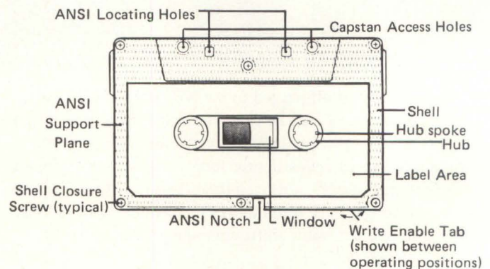
Digital Cassette: Front View
