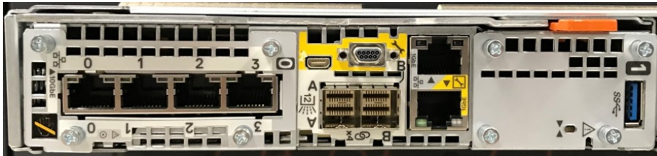
Figure 8 Embedded module with 10 GbE BASE-T 4-port card
