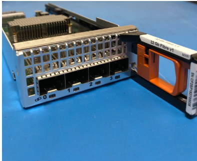
Figure 21 32 Gb Fibre Channel I/O module
