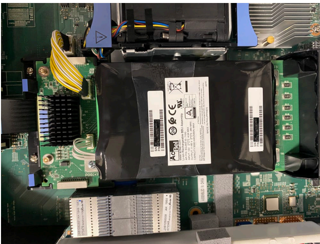
Figure 13 Battery backup unit
