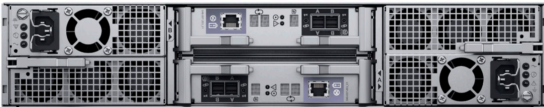
Figure 19 25-drive 2.5-inch 2U expansion enclosure (back)
