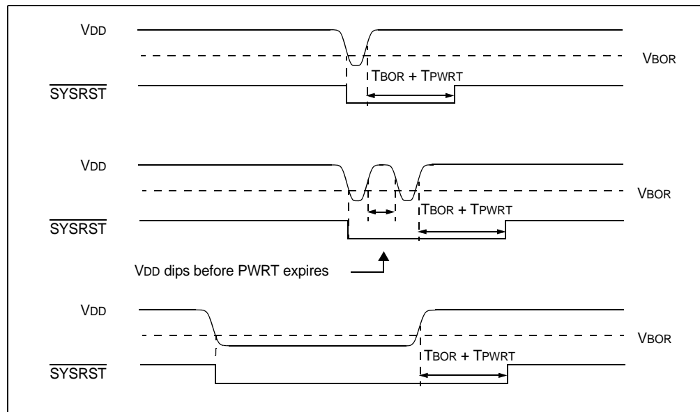
Figure 8-3: Brown-out Situations
