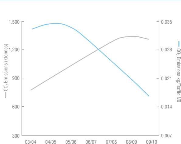
A forecast of the CO 2 emissions due to base stations, which account for 70% of the total network energy consumption
