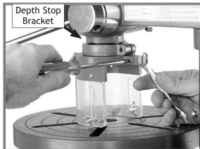
Figure 1. Example photo of installing chuck guard assembly.
