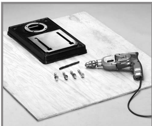
Figure 8. Secure base to plywood.
