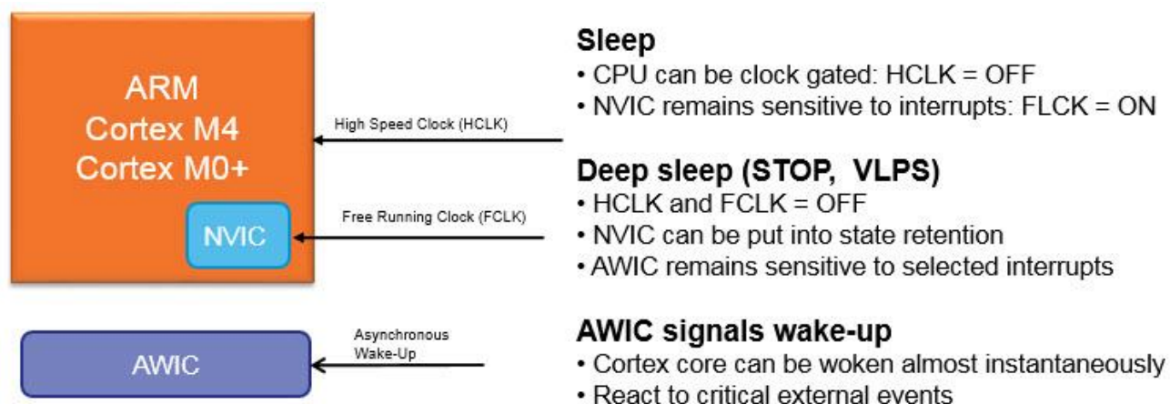
Figure 2. ARM Cortex M4 and M0+ architecture
