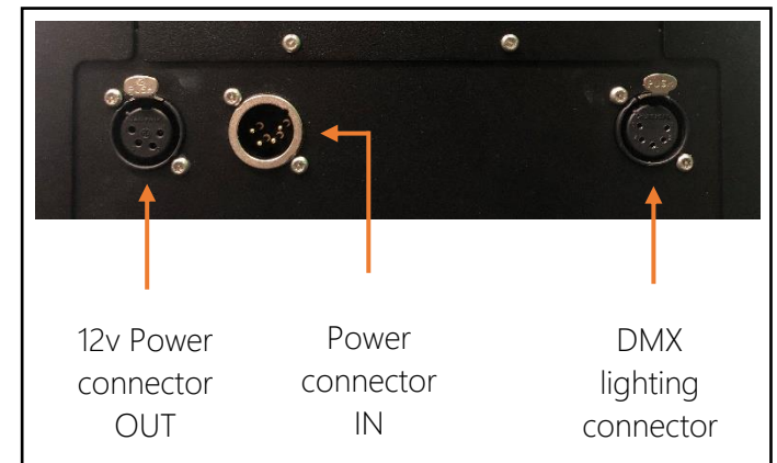
Rear bottom
