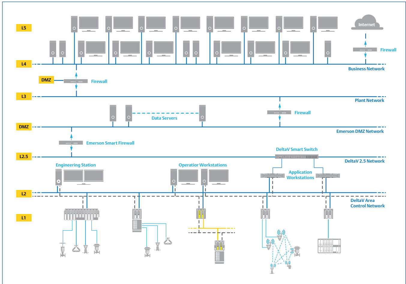
DeltaV reference architecture showing network segmentation and use of DeltaV Smart Switches in the 2.5 network.
