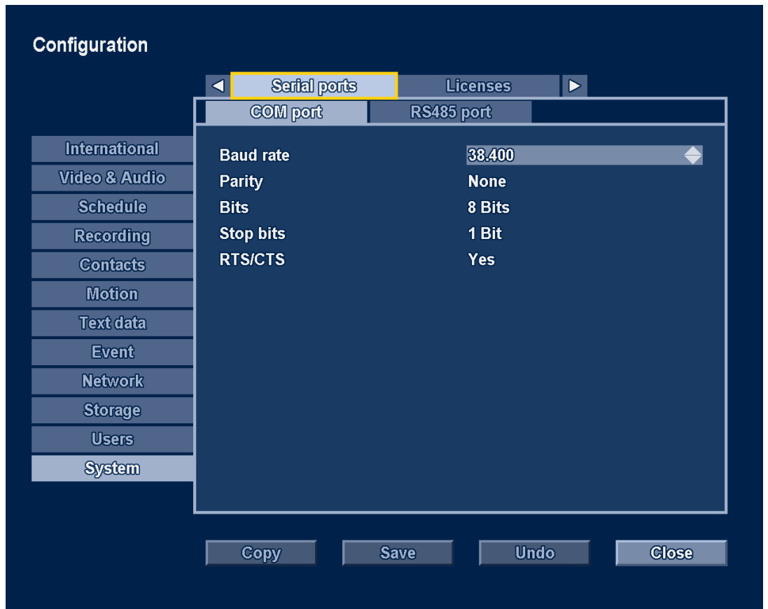
Figure 6.31 Configuration menu - System - Serial ports
