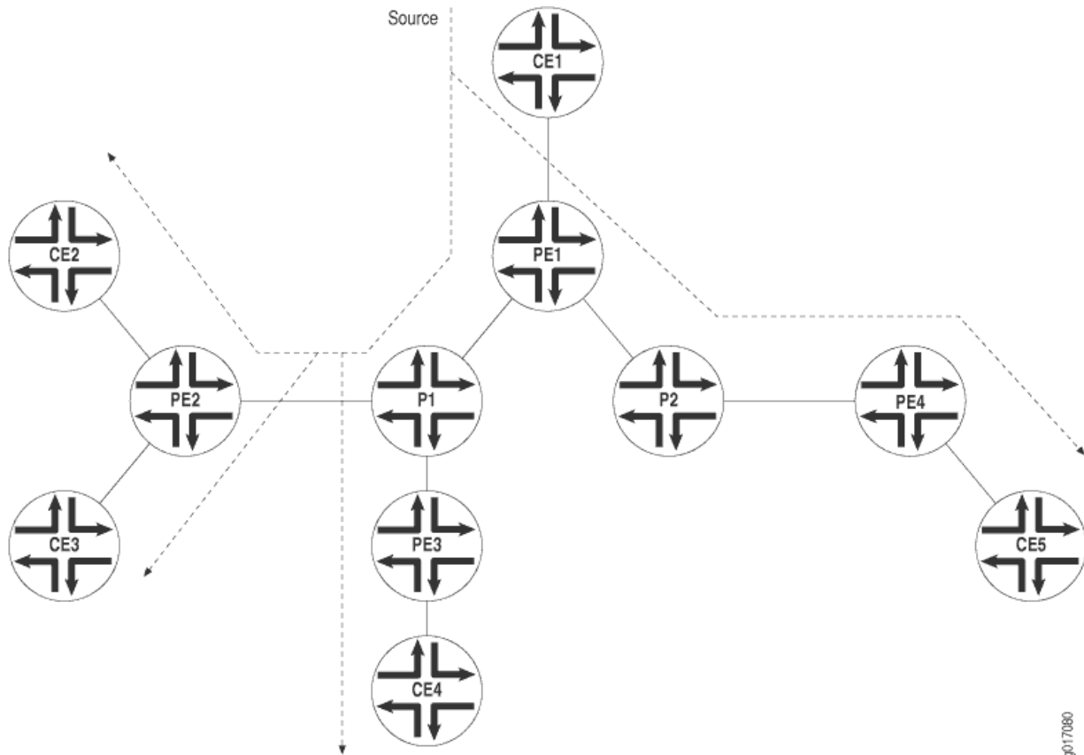
Figure 25: Point-to-Multipoint LSPs
