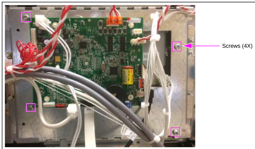
Figure 15: Loosening Phillips-head Screws
