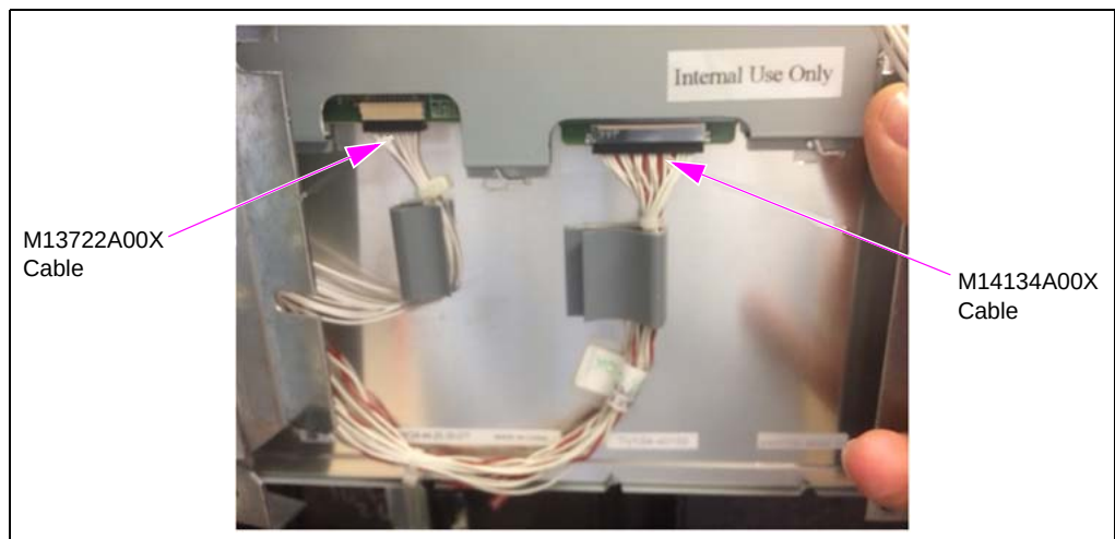
Figure 18: Attaching Cables
