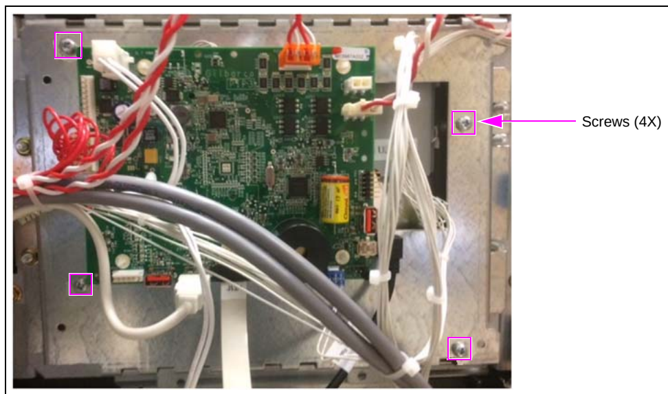
Figure 20: Tightening Phillips-head Screws
