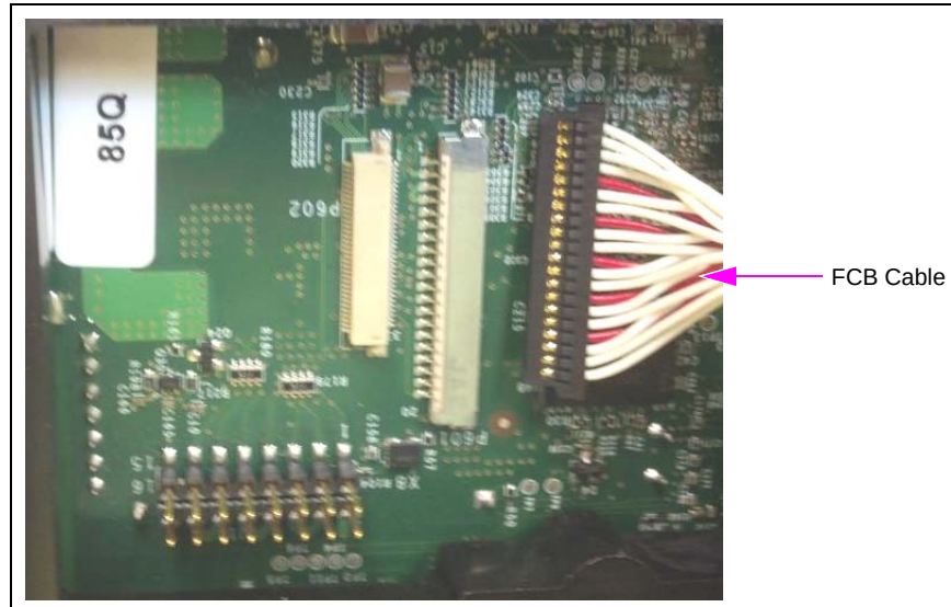
Figure 7: Positioning FCB Cable and P601
