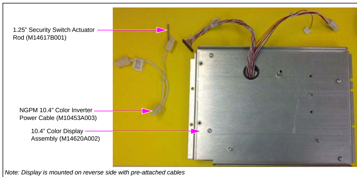
Figure 1: Kit Components
