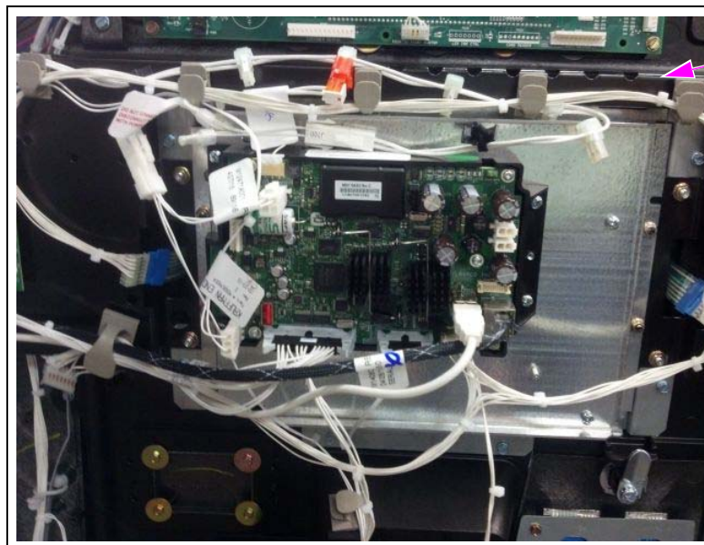
Figure 11: Assembly Mounted onto Dispenser
