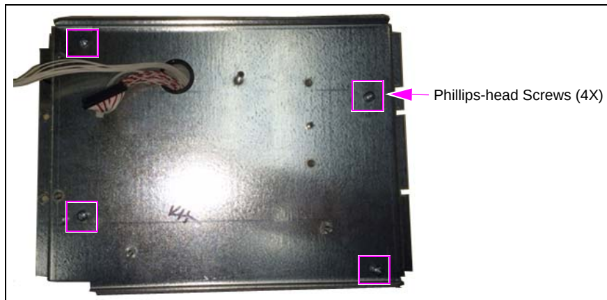
Figure 13: Removing Phillips-head Screws from Bracket
