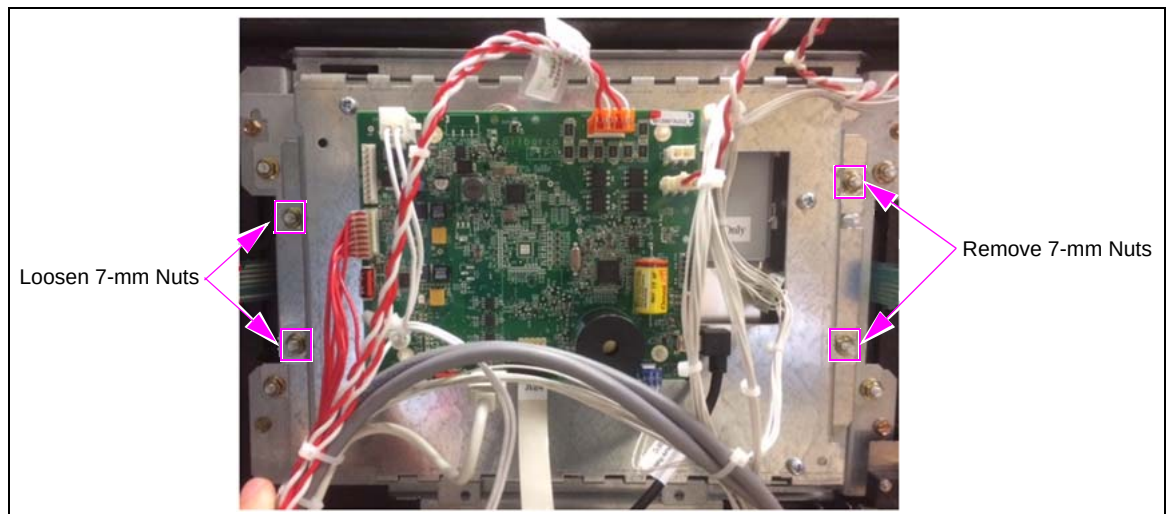
Figure 14: Removing 7-mm Nuts
