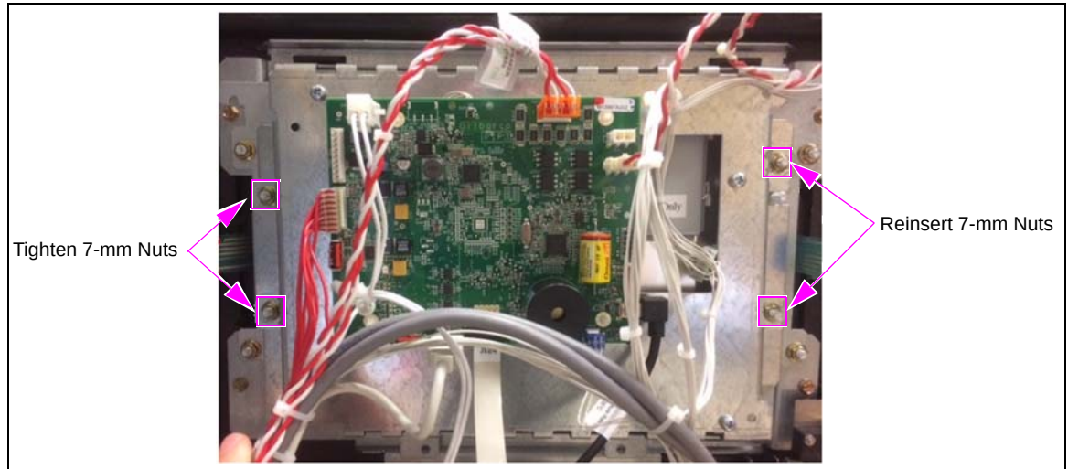
Figure 21: Tightening 7-mm Nuts
