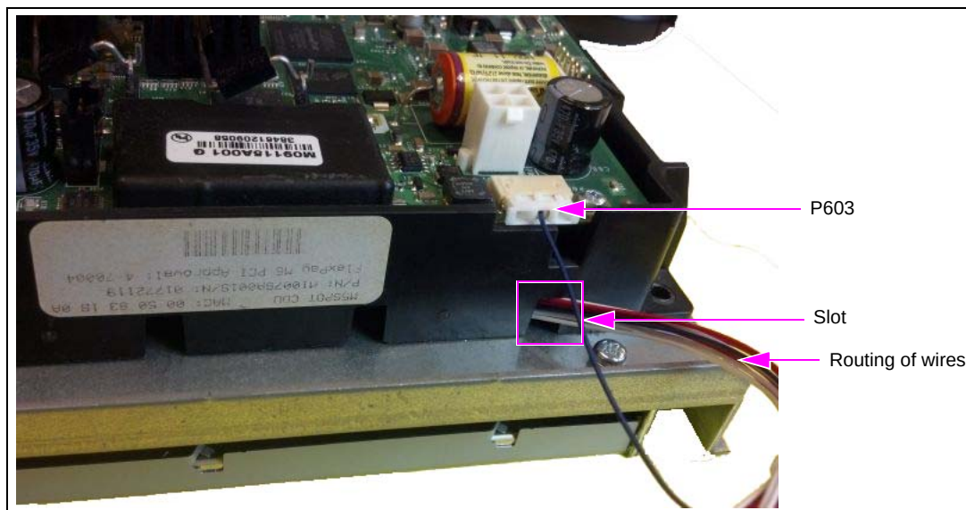
Figure 10: Connecting FCB to P603
