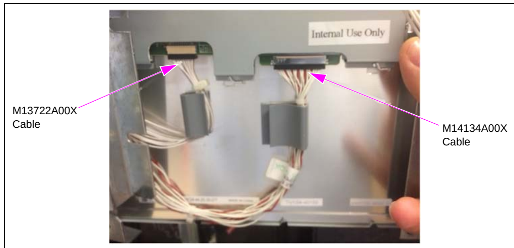
Figure 17: Detaching Cables
