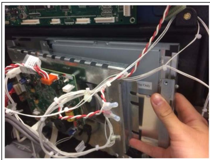
Figure 16: Removing 10.4-inch Screen from Door
