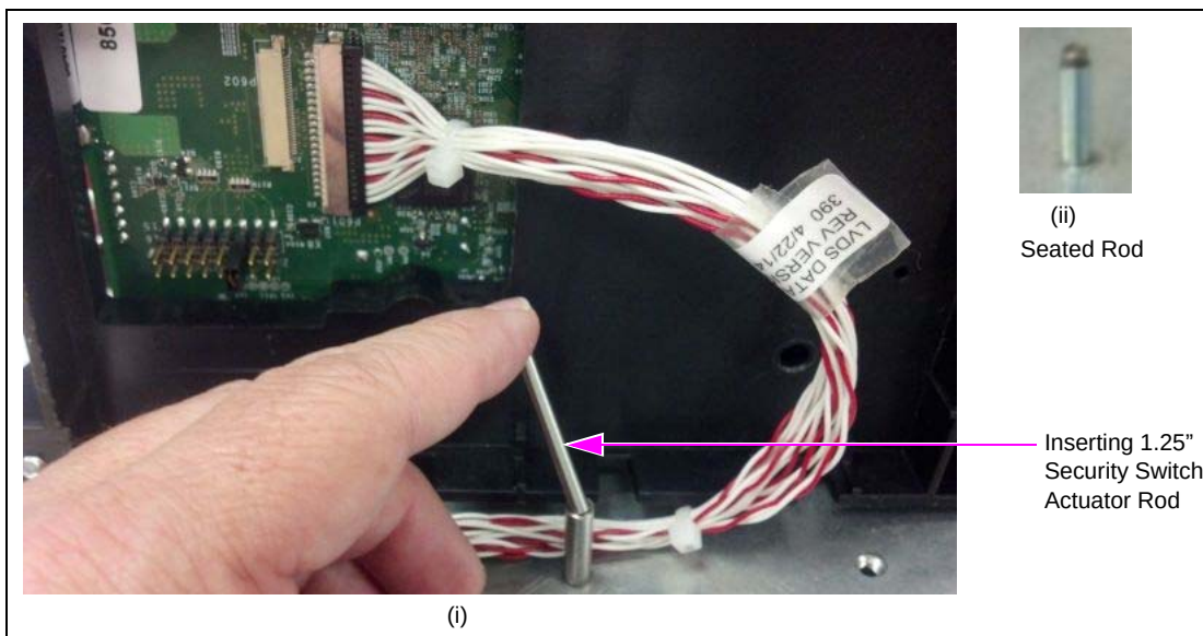
Figure 9: Inserting Security Switch Actuator Rod (M14617B001)
