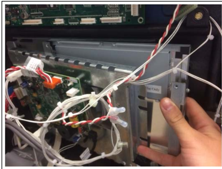
Figure 19: Mounting 10.4-inch Screen to Door
