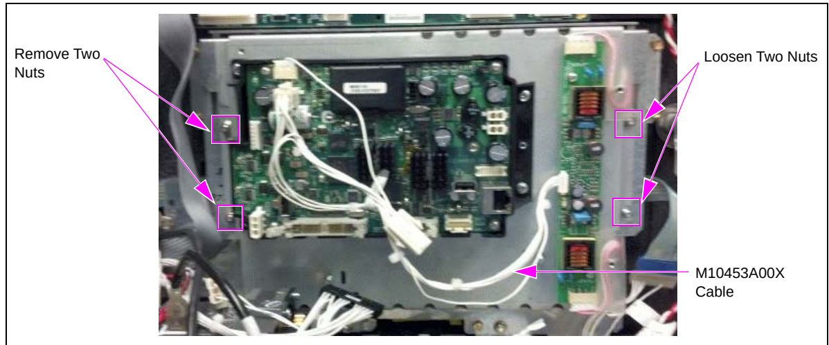
Figure 3: Removing FCB/Display Assembly
