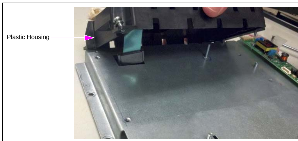
Figure 5: Tilting Plastic Housing
