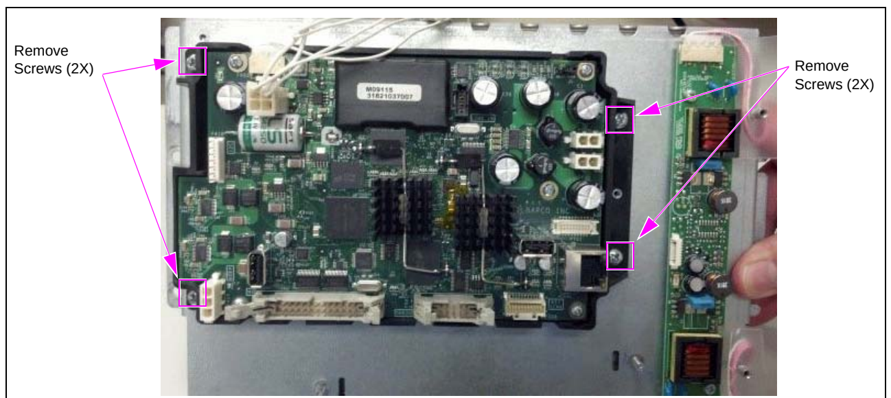
Figure 4: Removing Board and Plastic Housing
