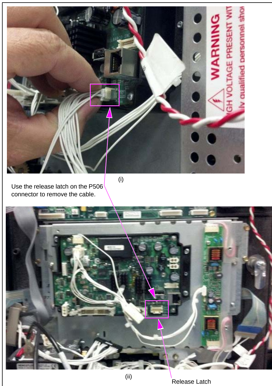
Figure 2: Removing Cables
