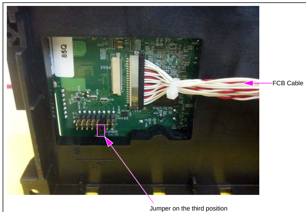
Figure 8: Connecting FCB Cable and P601
