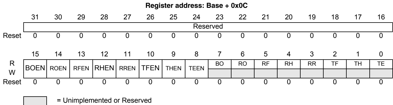
Figure 39. Interrupt Control/Status Register (INTREG)
