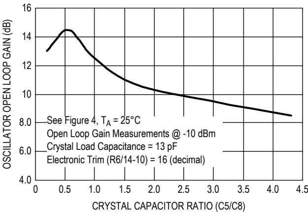
Figure 21. Oscillator Open Loop Gain vs. Capacitor Ratio
