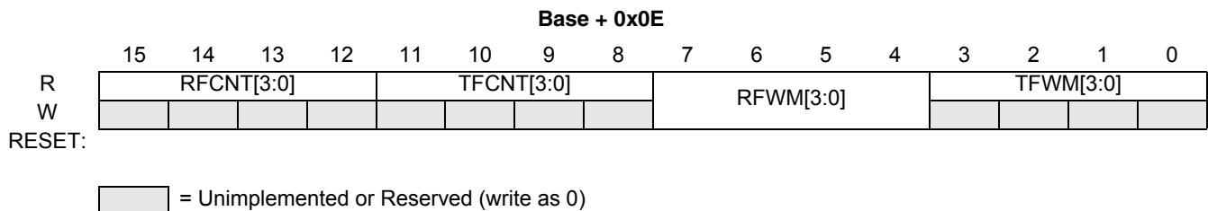
Figure 63. SFCSR Register Diagram
