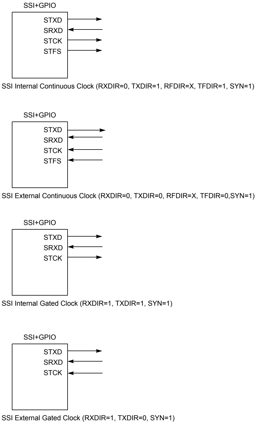
Figure 50. Synchronous SSI Configurations—Continuous and Gated Clock
