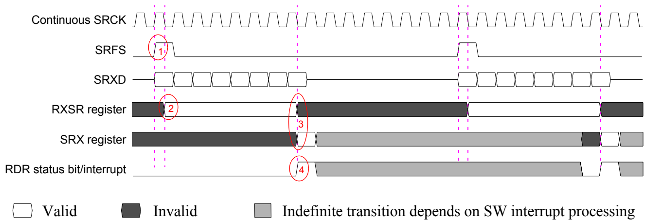
Figure 72. Normal Mode Receive Timing—Continuous Clock (WL=8-bit words, DC=1)
