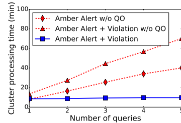
Figure 12: As the number of queries scale, query optimization ensures that the cluster processing time for both sets of queries stays constant by using auto-parallelization and de-duplication.
