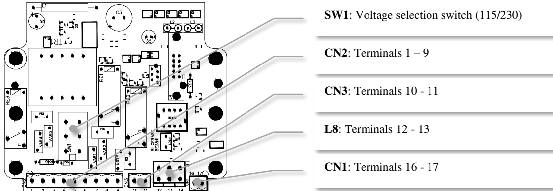
Illustration 4: Base PCB of 115/230 VAC MASTER unit.
