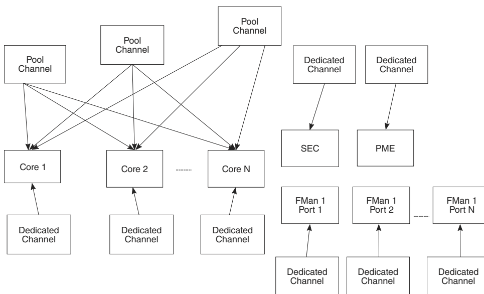
Figure 66. DPAA1 Channel Types
