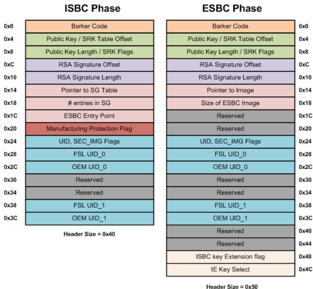
Figure 26. CSF Header for LS1 (ISBC and ESBC Phase)
