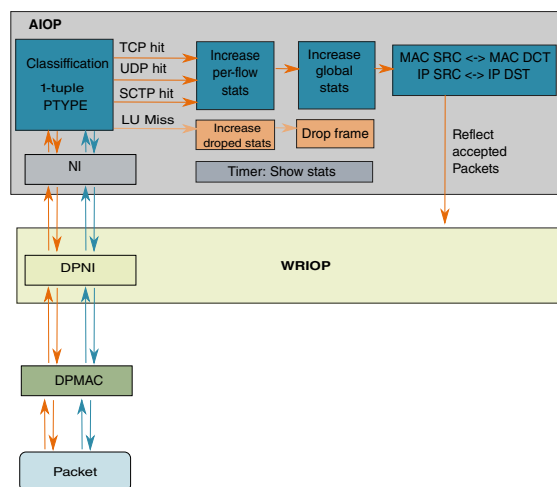
Figure 170. AIOP Statistics overview
