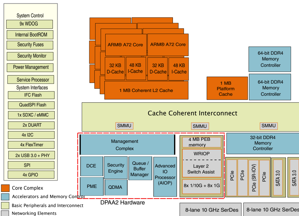
Figure 136. LS2088A SoC
