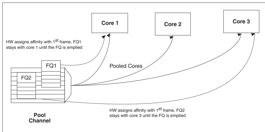
Figure 72. Hold Active Scheduling
