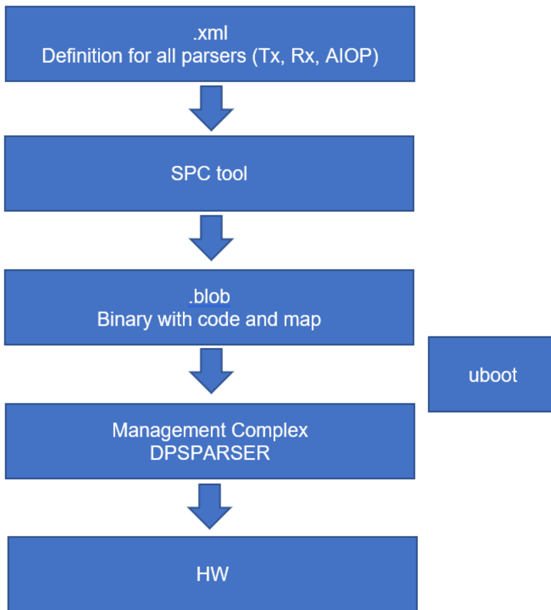
Figure 160. High-level solution overview
