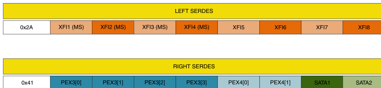
Figure 155. SERDES
