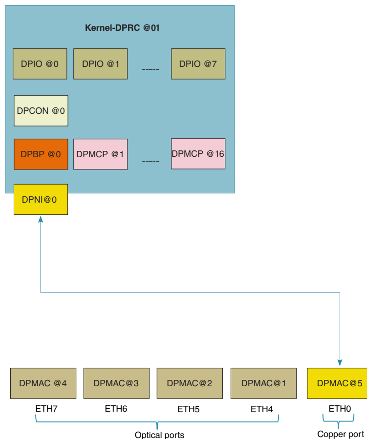
Figure 156. RDB DPL container configuration
