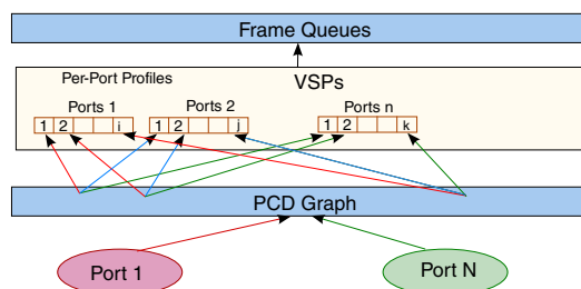
Figure 118. FMan PCD graph and the VSP selection
