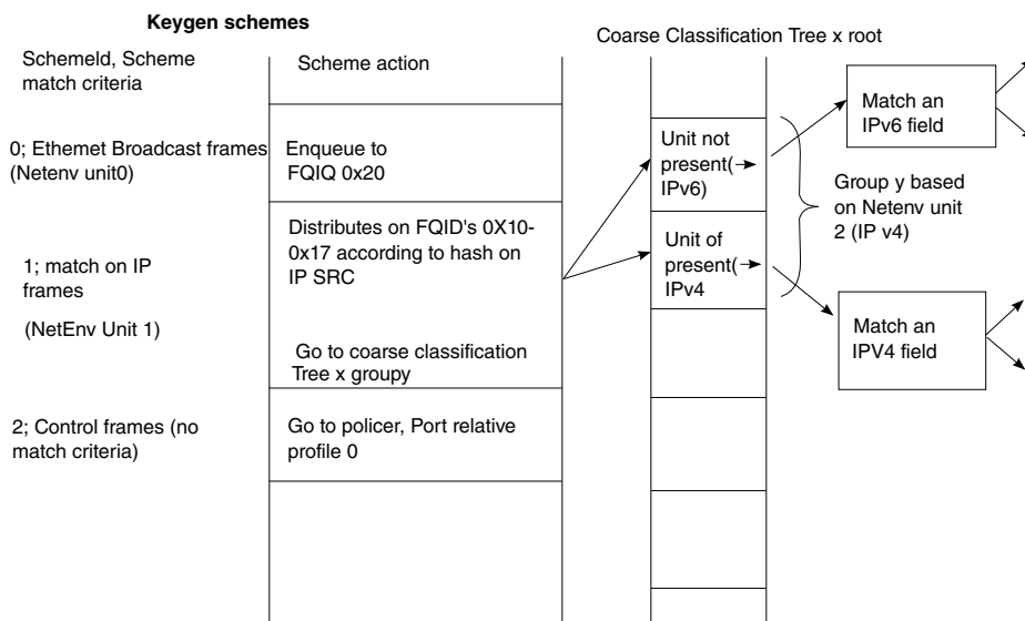
Figure 110. Keygen -> Custom Classifier Example
