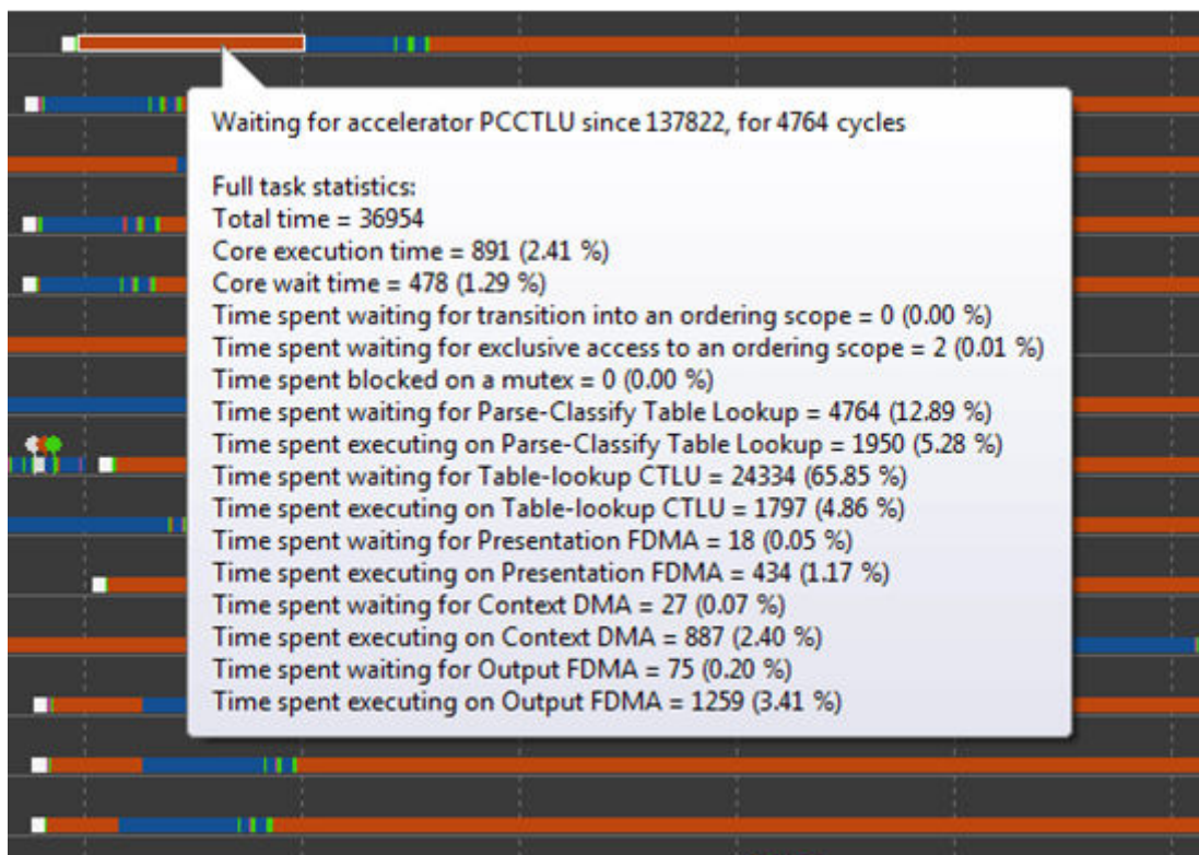
Figure 184. CTLU - Parser Bottleneck Example
