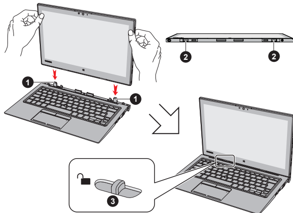
Figure 2-4 Docking the tablet computer
