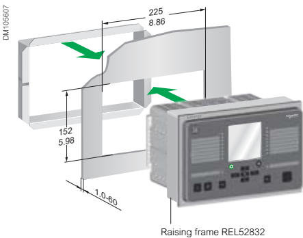
Projection mounting with the raising frame REL52832
