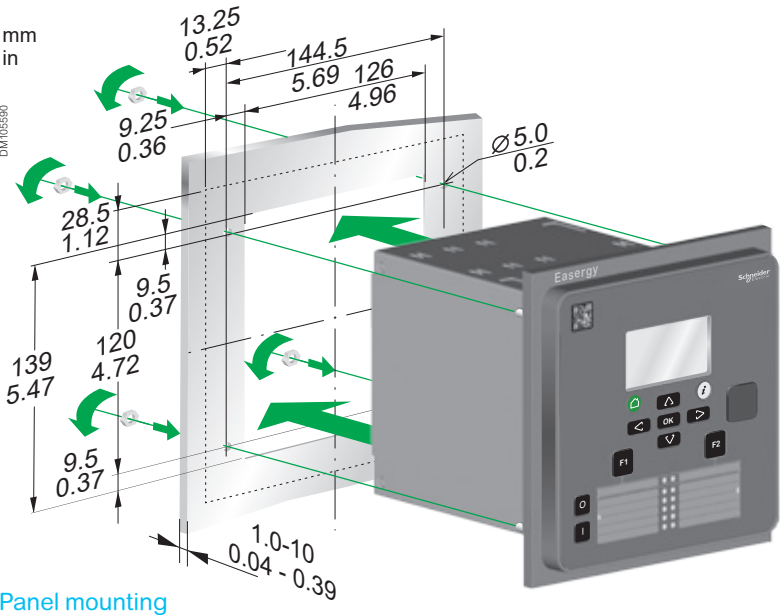
Panel mounting
