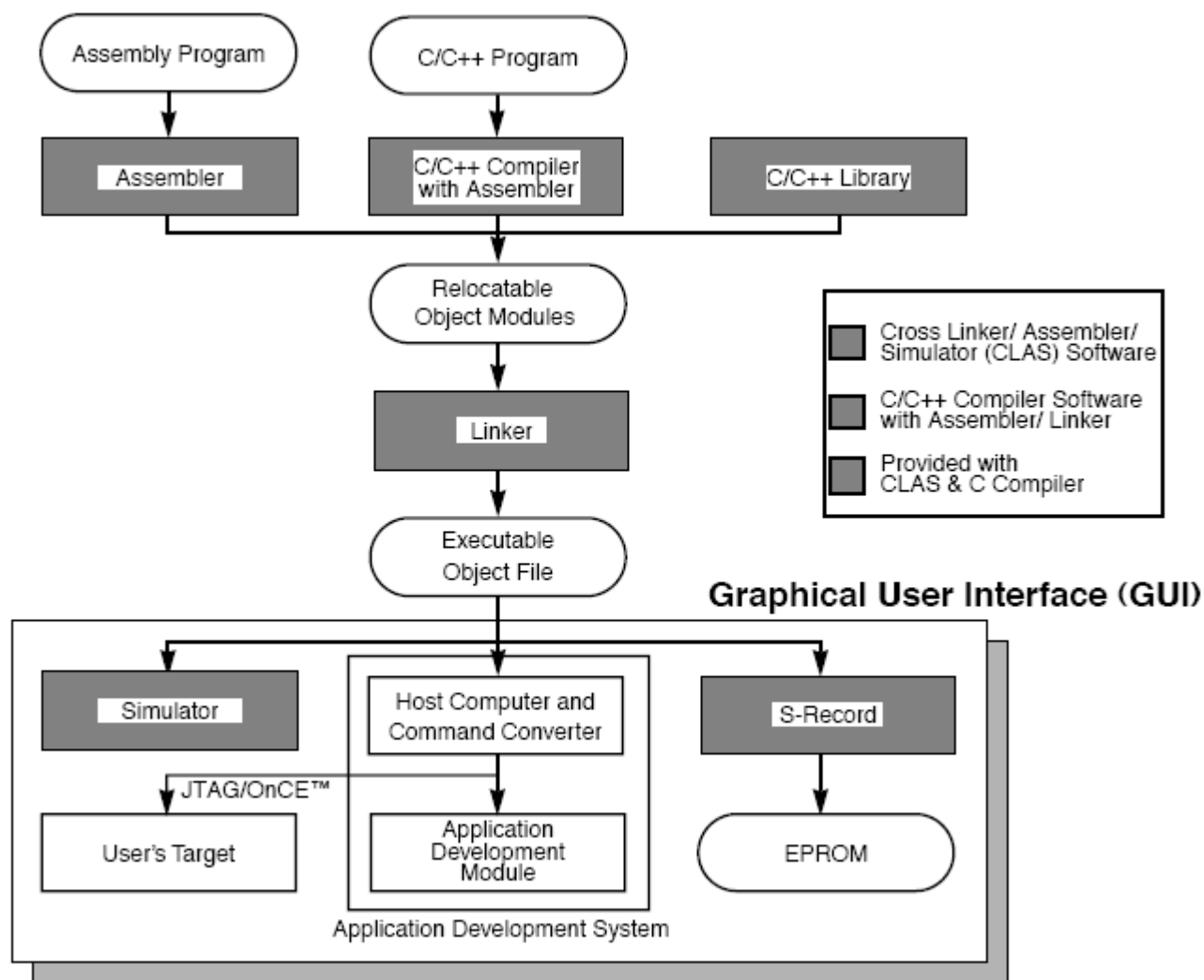
Figure 11-2. Development Flow
