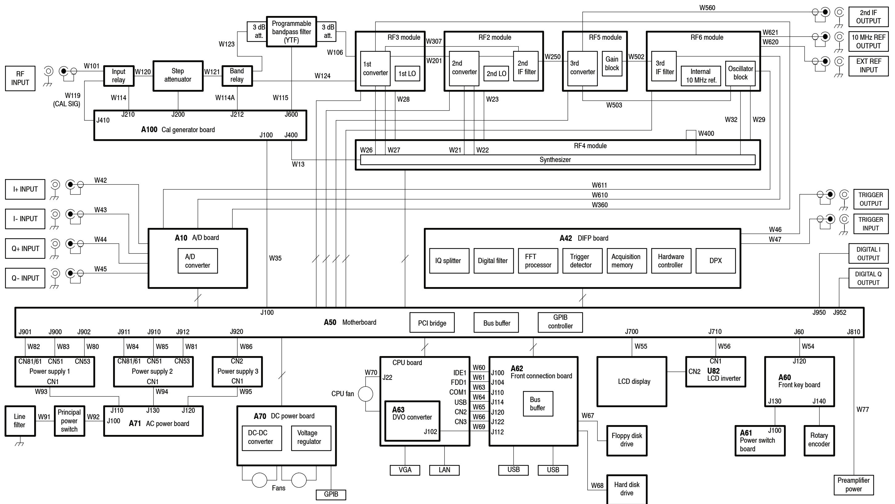
Figure 6-2: Interconnect diagram
