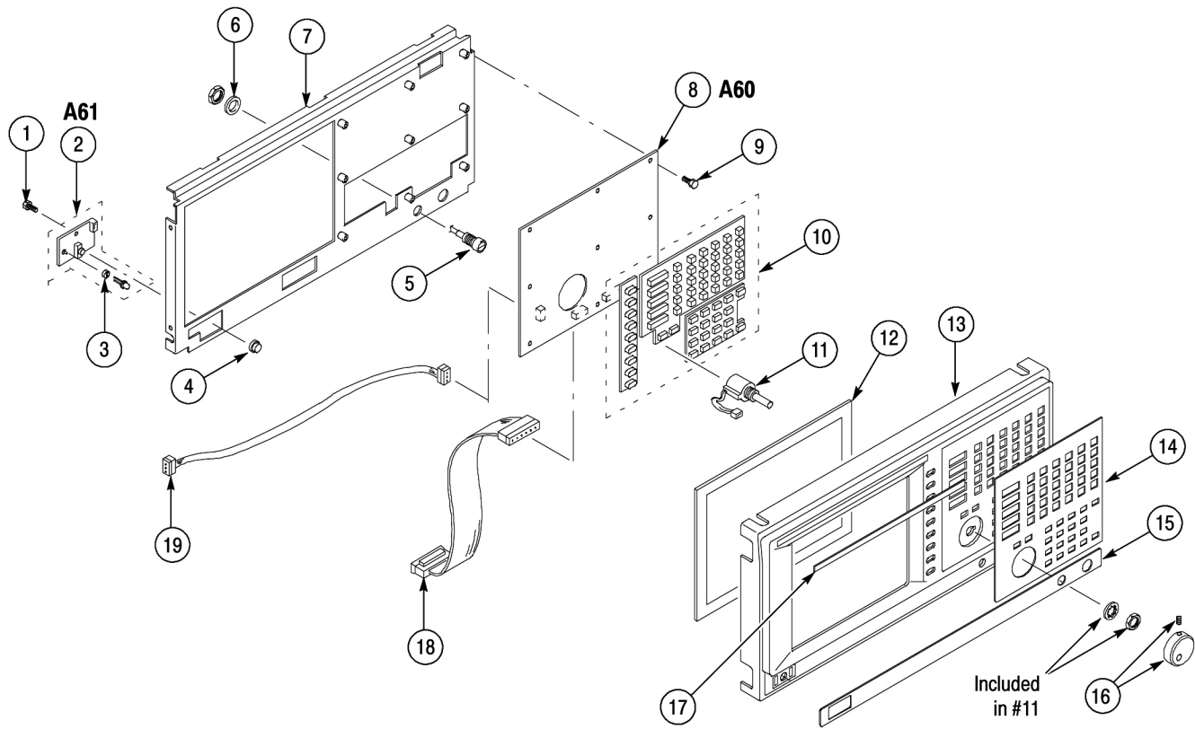
Figure 7-2: Front-panel assembly - 1
