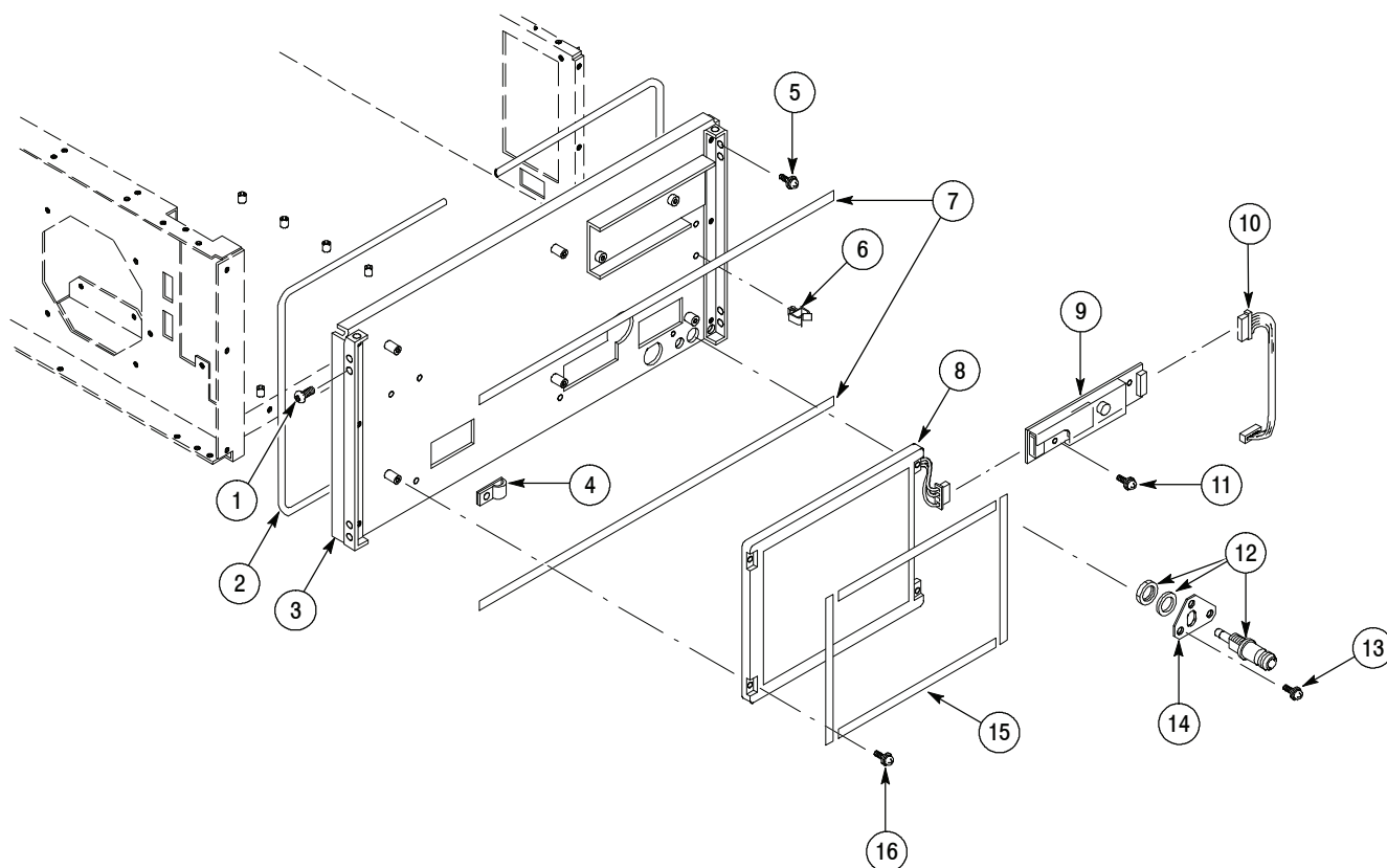
Figure 7-3: Front-panel assembly - 2
