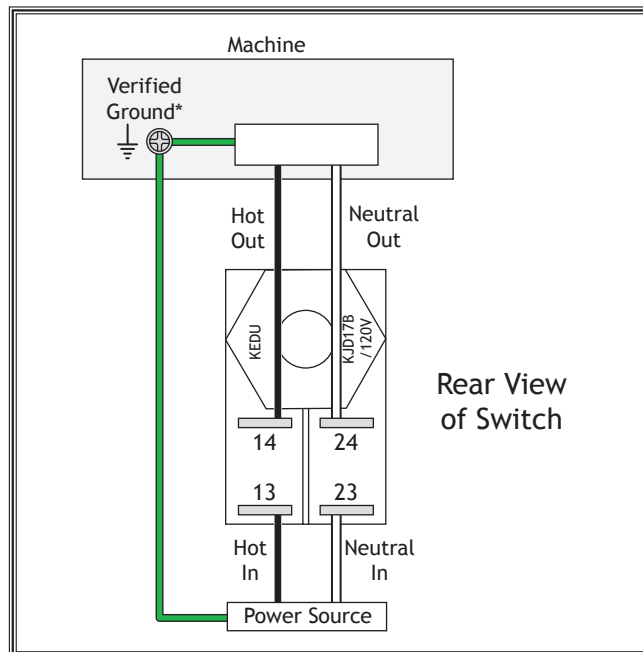
Figure 2. D4160 wiring diagram.
