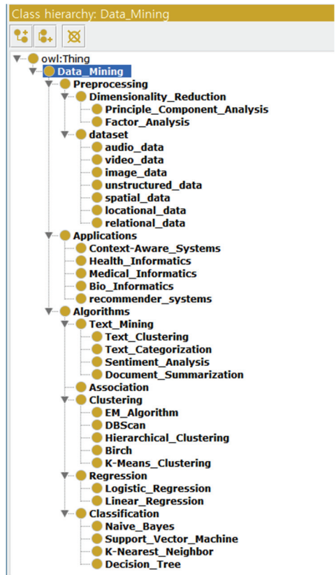
Fig. 2. Class Hierarchy in UniDM ontology.
