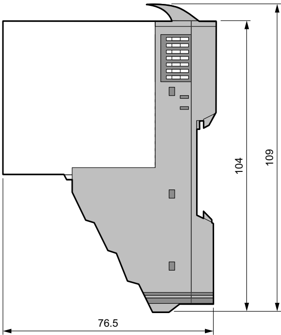
Peripheral module
