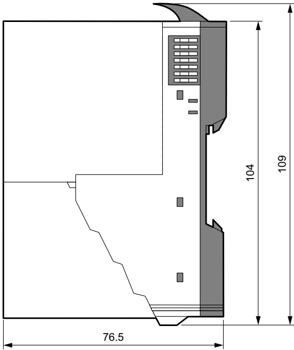
Bus coupler
