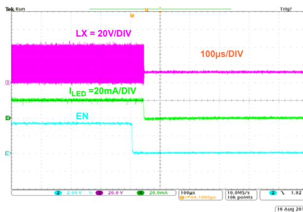
FIGURE 19. ISL97672B SHUTS DOWN AND STOPS SWITCHING ~30μs AFTER EN GOES LOW
