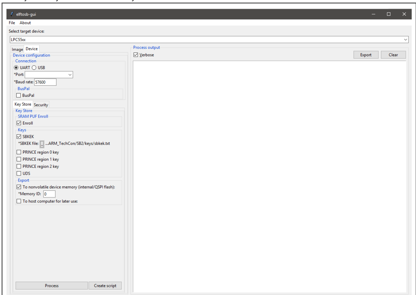
Figure 13. ELFTOSB-GUI setup for SBKEK load
