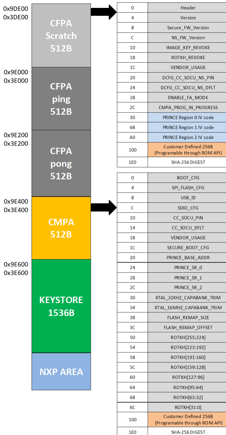
Figure 8. Protected flash region LPC55xx family
