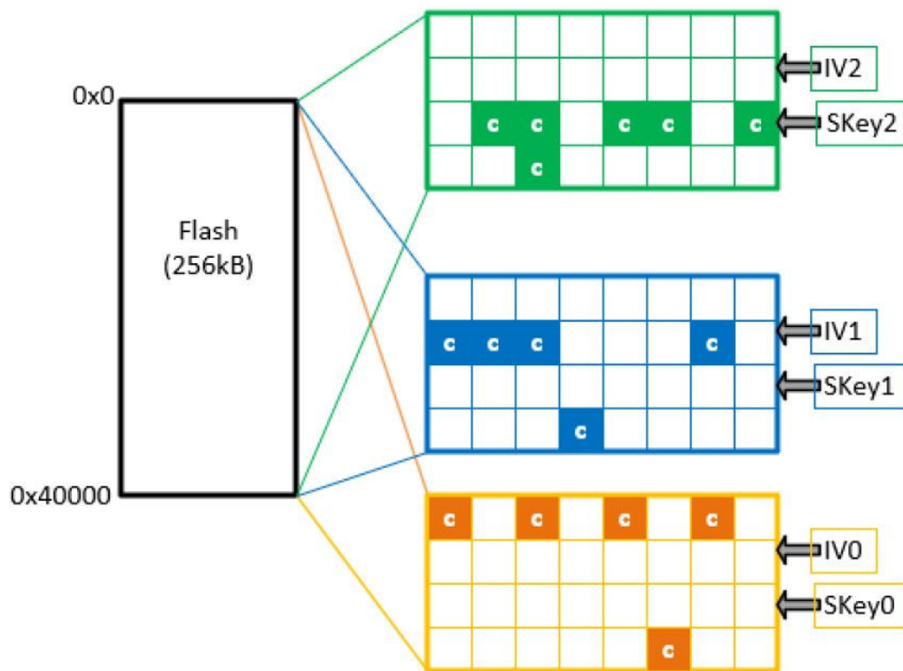
Figure 7. PRINCE regions in LPC55S1x and LPC55S0x
