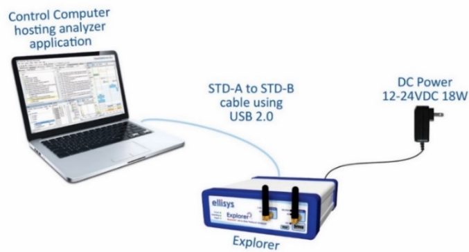
Figure 9 Basic Setup for Explorer (USB and DC PWR)
