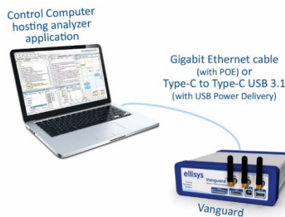
Figure 12 Basic Setup for Vanguard using a Direct Connection (Ethernet or USB)
