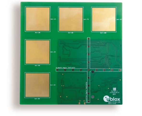
Figure 1: u-blox direction-finding explorer kits comprising C211 application board(s) and C209 tag(s)
