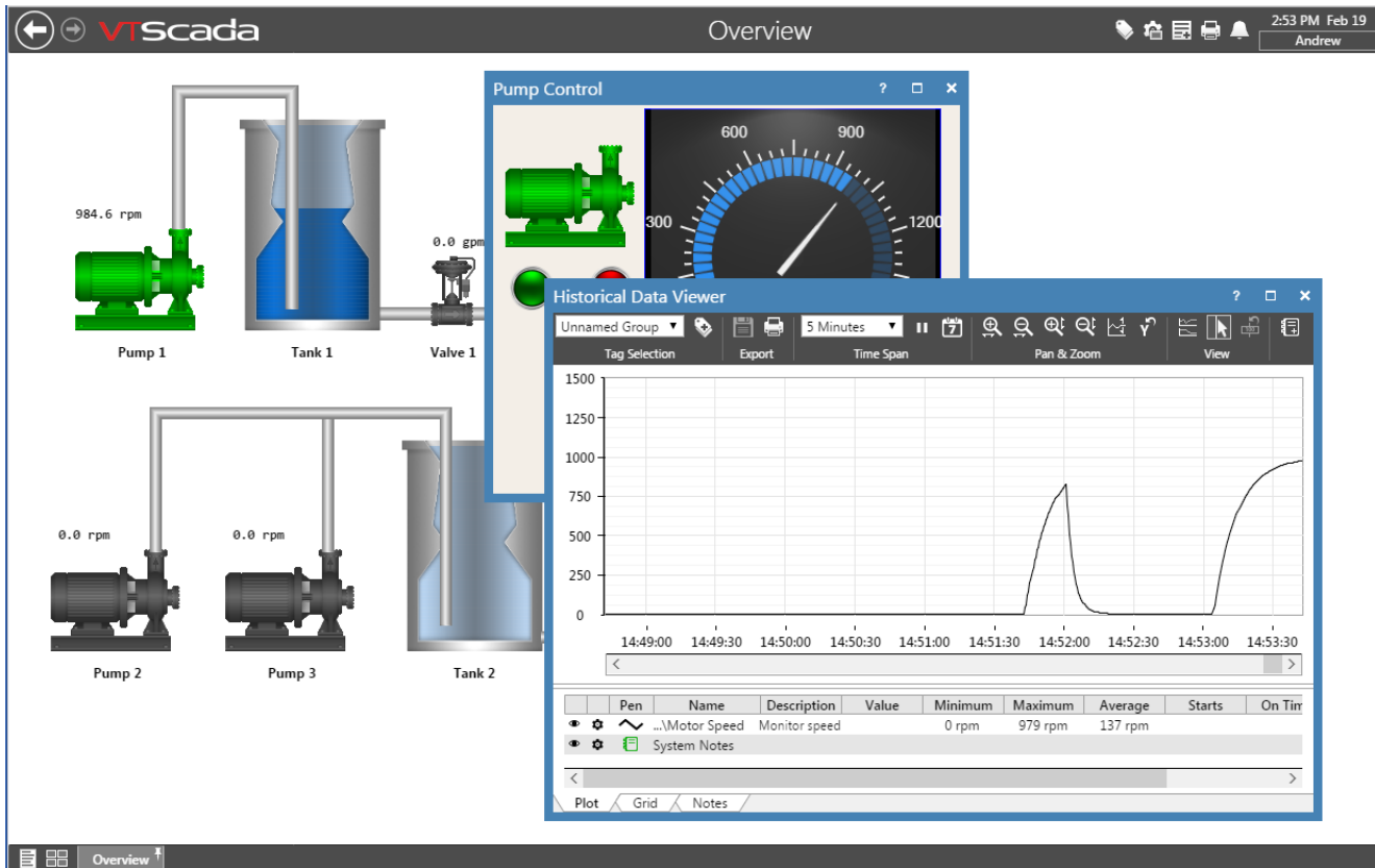
The Completed Tutorial application, with a pop-up window and a trend, running in Chrome using the Anywhere Client.
