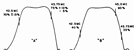
Figure 7—Mixer Plate and Overall I.F. Response
