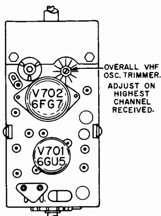
VHF Channel Adjustment Location.
