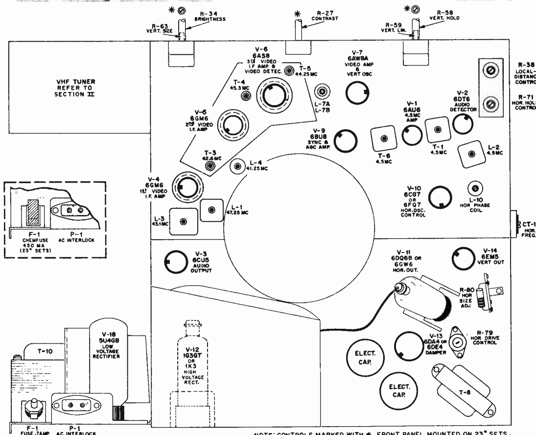
TUBE LOCATION AND ALIGNMENT POINTS
