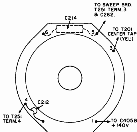
YOKE WIRING
