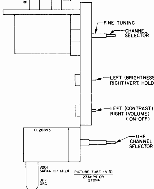
TUNE & TRIMMER LAYOUT - MB & MBU CHASSIS
