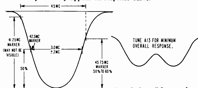
Figure C. Ideal IF Response Curve.
