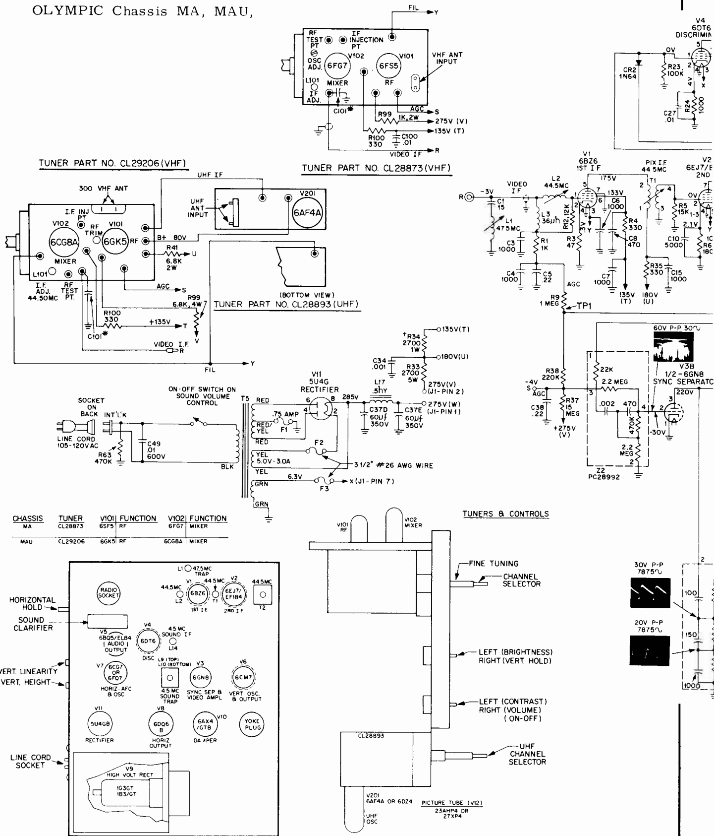
TUBE & TRIMMER LAYOUT - MA & MAU CHASSIS
