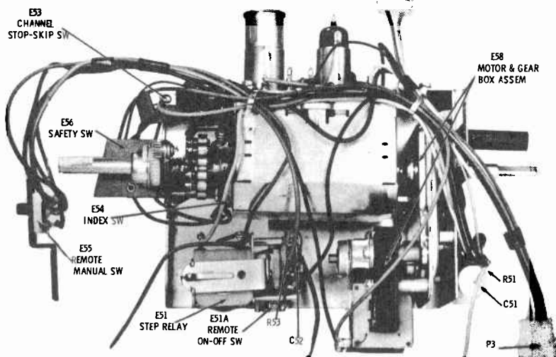
AUTOMATIC TUNER
