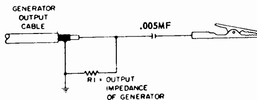
Figure 8 - Generator Cable Termination.
