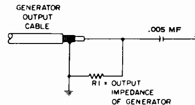
Figure 13 - Generator Cable Termination
