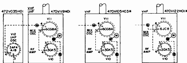
Figure 3 - Rear View.
