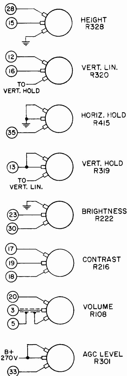
Control Wiring Diagram. All Views Seen From Rear.
