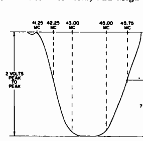
Figure 15 - Response, Mixer Grid to 2nd Det
