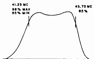
Figure 6—T208 3rd Pix-I.F. Response
