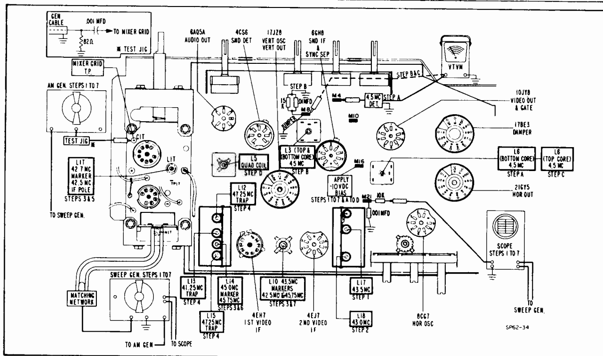
13G20 Equipment Setup &amp; Alignment Points
