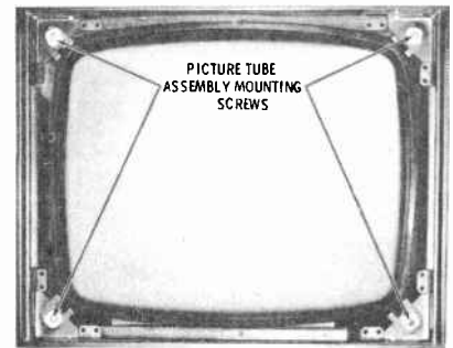
MODEL 23K90 CRT MOUNTING FRONT VIEW
