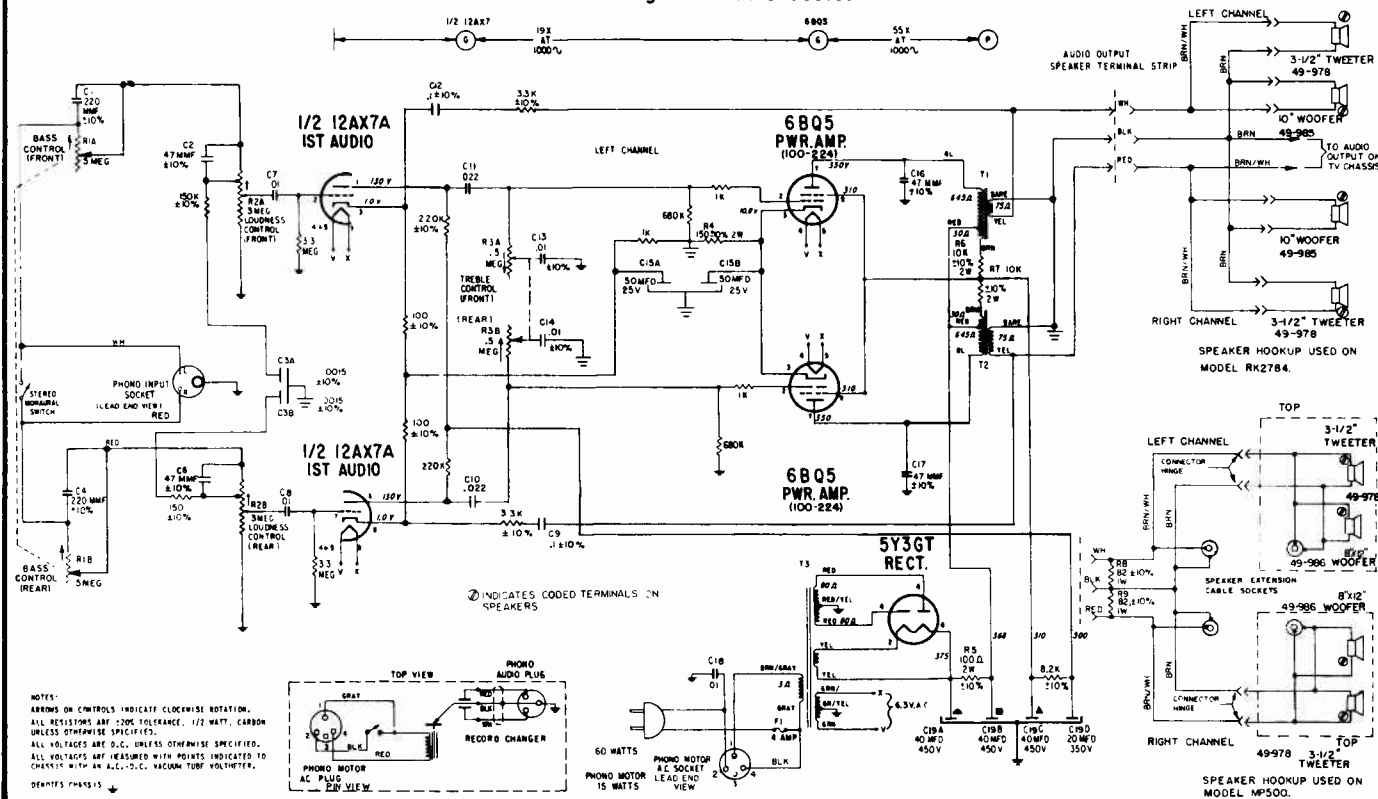
Schematic Diagram 4K22 Chassis.
