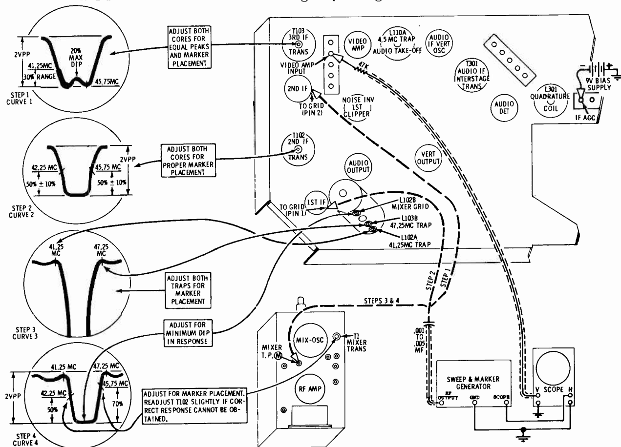
VIDEO IF &amp; SOUND ALIGNMENT DETAIL
