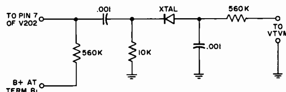
Figure 10—Sound Diode Detector
