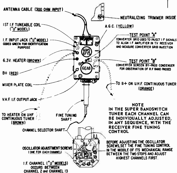
Fig. 1. Tube and Trimmer Layout, Bandswitch Tuner.
