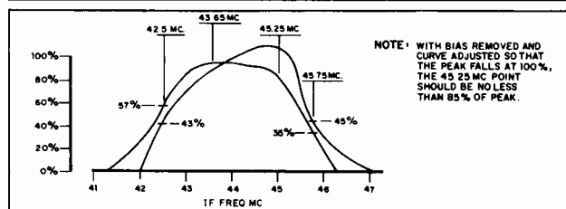
Figure I-7. Overall I-F Response Curve 13J27 and 13J28 Chassis
