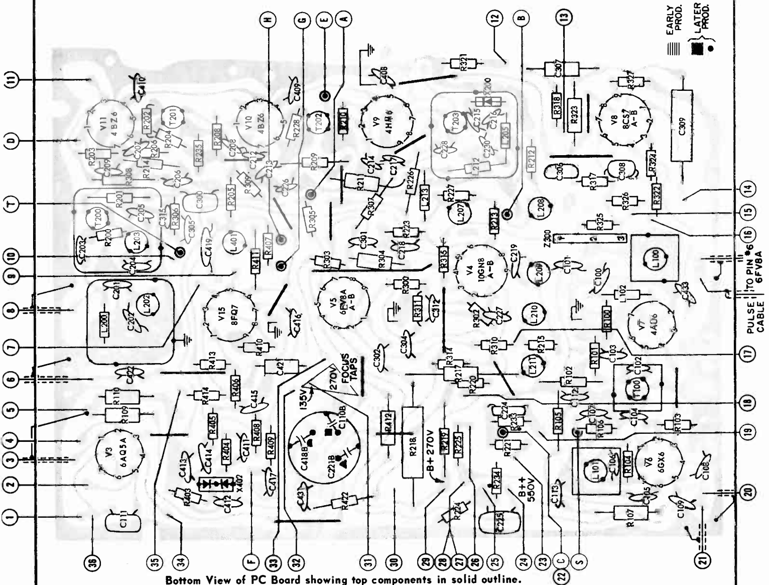
Bottom View of PC Board showing top components in solid outline. Tube pin numbering is for bottom of socket.
