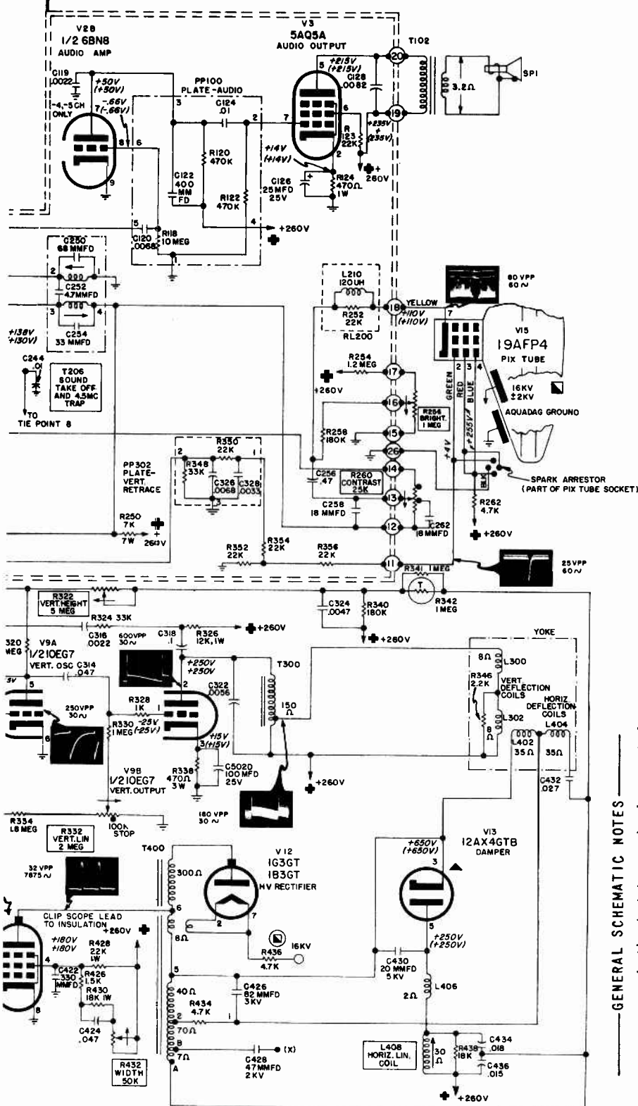
SCHEMATIC DIAGRAM (563-1,-2,-4,-5,-7)
