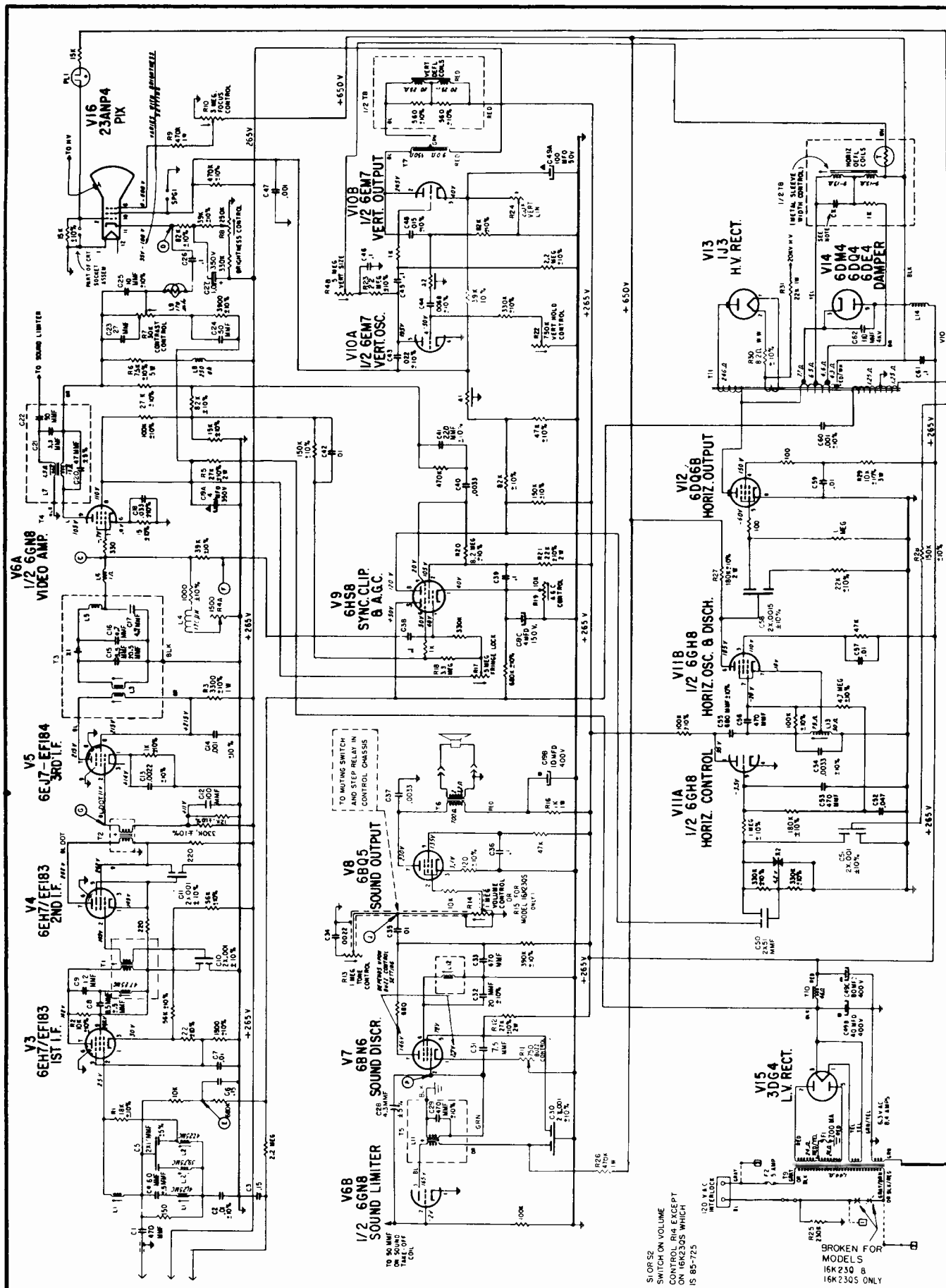
Schematic Diagram 16K23, 16K23Q and 16K23QS Chassis.
