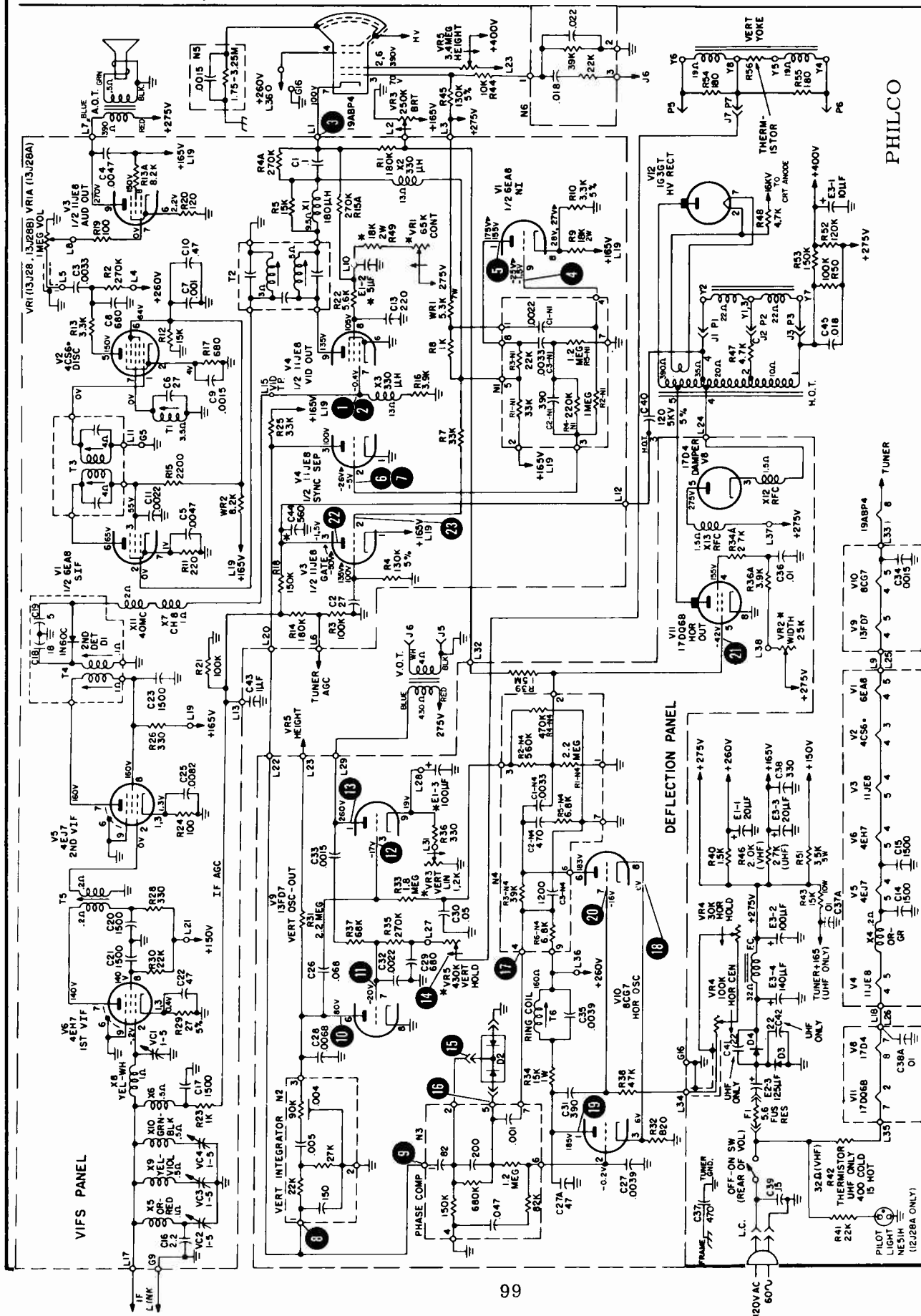
13J28 Schematic Diagram
