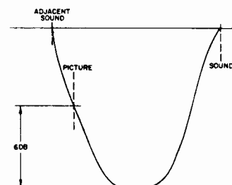
Figure 14 - Typical RF-IF response.
