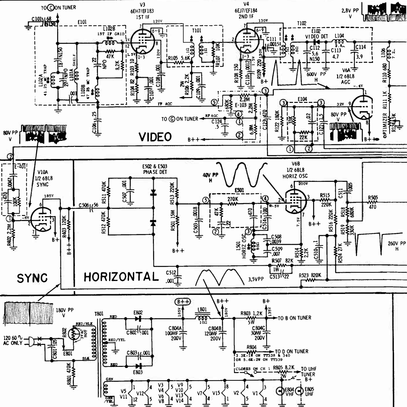
T501 CONN
