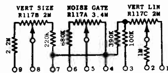
R117 CONN DETAIL
