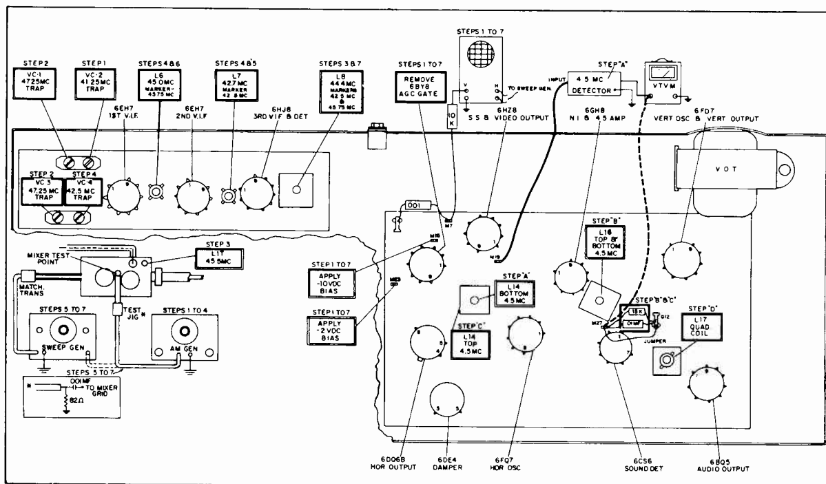
Equipment Set-Up and Alignment Points - 13N50, 13N51, 13N52 &amp; 13N53 Chassis
