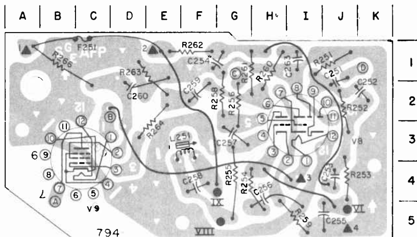
SWEEP BOARD SOLDER SIDE
