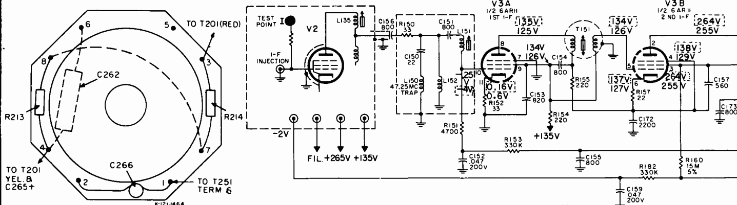
YOKE WIRING
