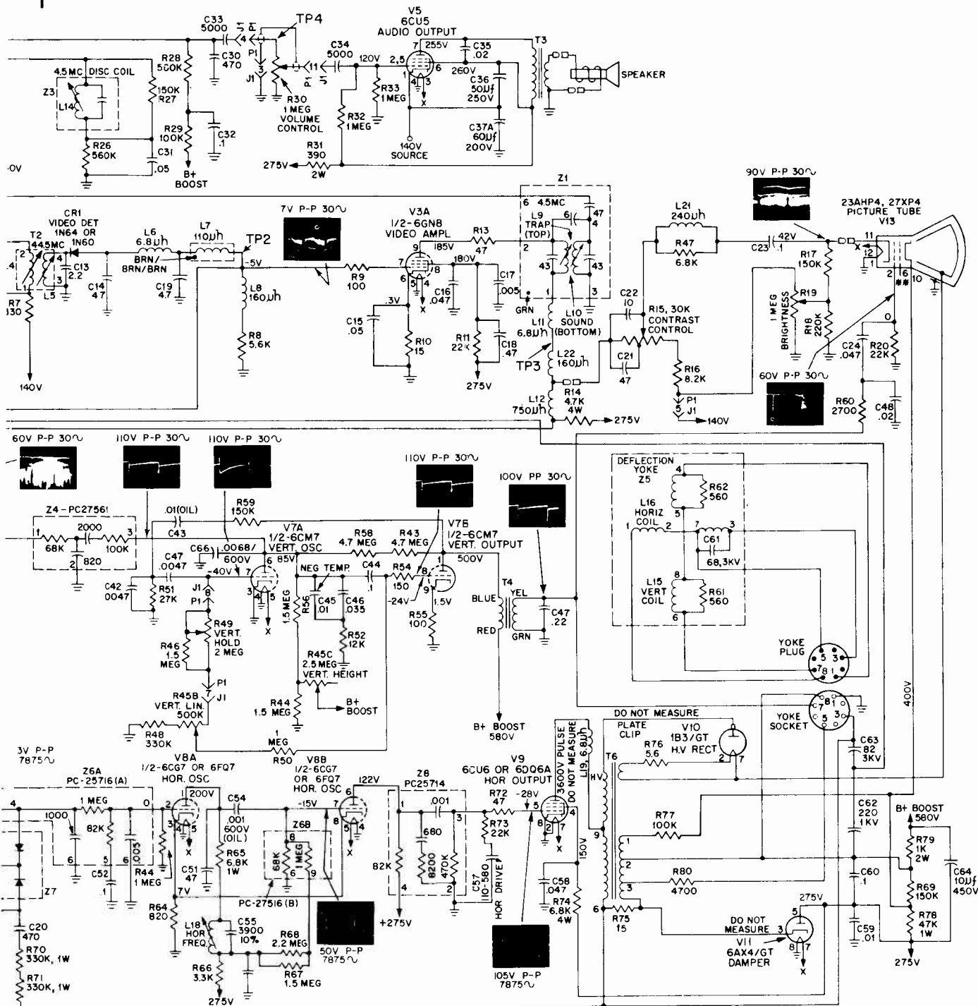
CHASSIS MB & MBU, SCHEMATIC DIAGRAM
