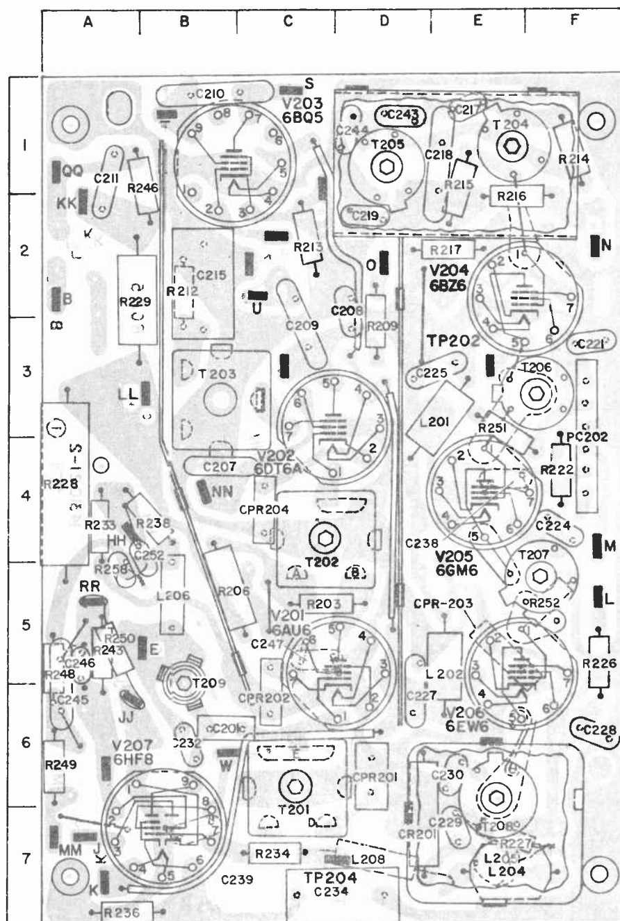
Figure 13—PW200 Sealed Circuit L.F. and Video Assembly Composite Diagram
