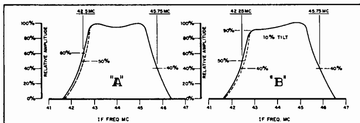
FIGURE 1-8A Overall I-F Response Curves 13J41, 13J42, 13J43 and 13J45 Chassis
