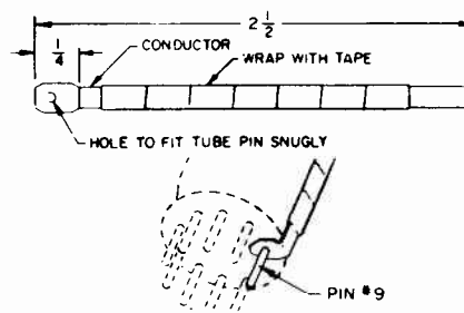
Figure 10 - Mixer Coupling Device.
