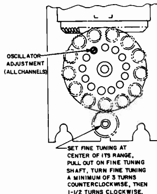
Figure 3—One-Set Fine Tuning—Remote
