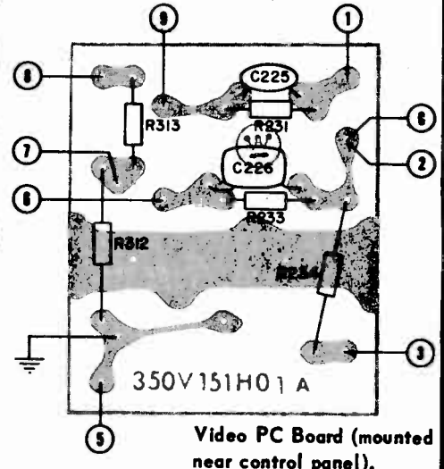
Bottom view of PC Board, showing top components in solid outline. Tube pin numbering is for bottom of socket.
