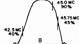
Figure 8—Mixer Plate and Overall I-F Response
