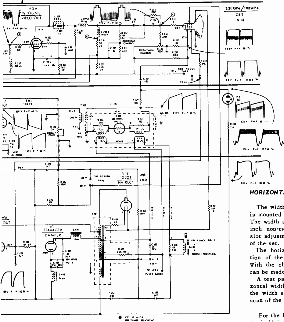
Schematic Diagram of Chassis V-2435-1 thru -11. Figure 7
