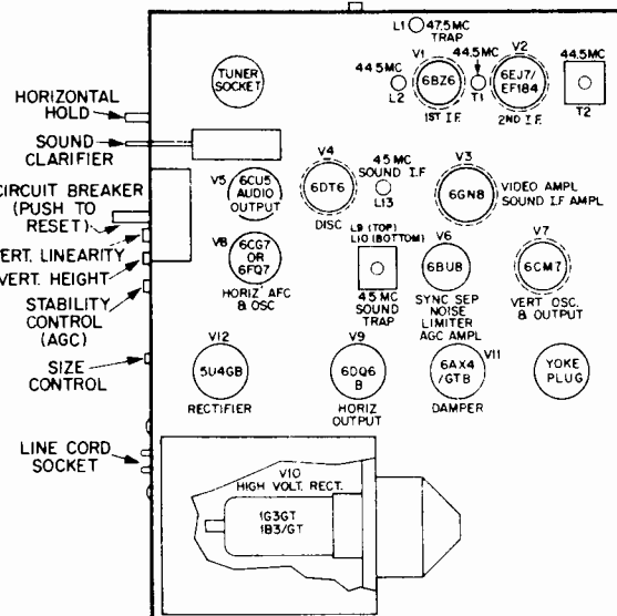
TUNE & TRIMMER LAYOUT - MB & MBU CHASSIS
