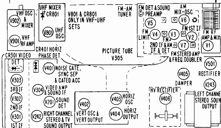
TUBE LOCATIONS
