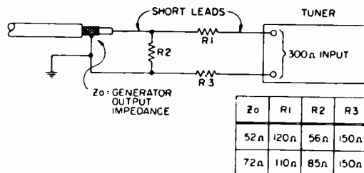
Figure 12 - Impedance Matching Network
