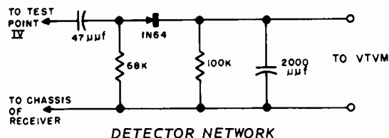
DETECTOR NETWORK
