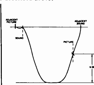
Figure 16 - Typical RF-IF Response
