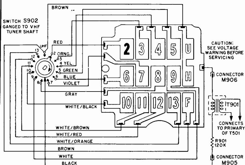
Circuitry of Dialescent Panel and Switch Assembly in Models with 21C4 or 21UC4 Chassis.
