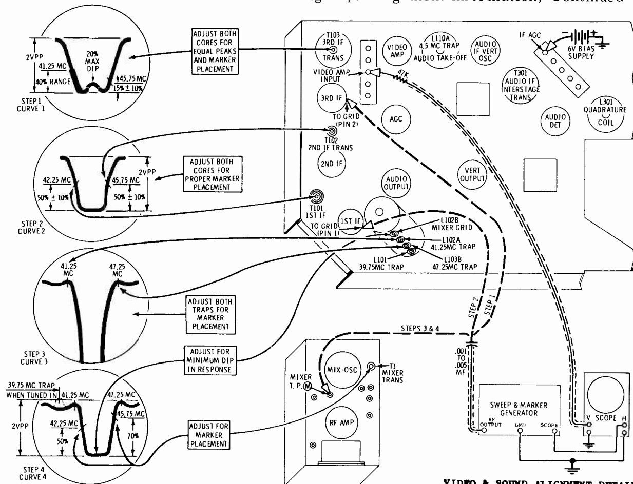
VIDEO &amp; SOUND ALIGNMENT DETAIL
