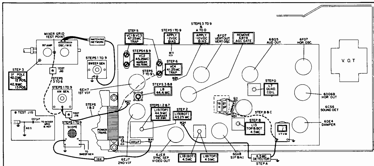
Equipment Set-Up and Alignment Points - 13J41, 13J42, 13J43 & 13J45 Chassis
