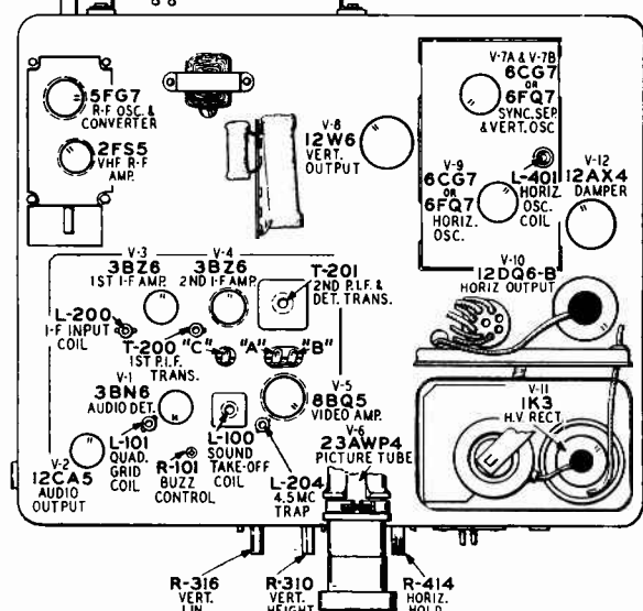
Chassis Tube Layout and Trimmers
