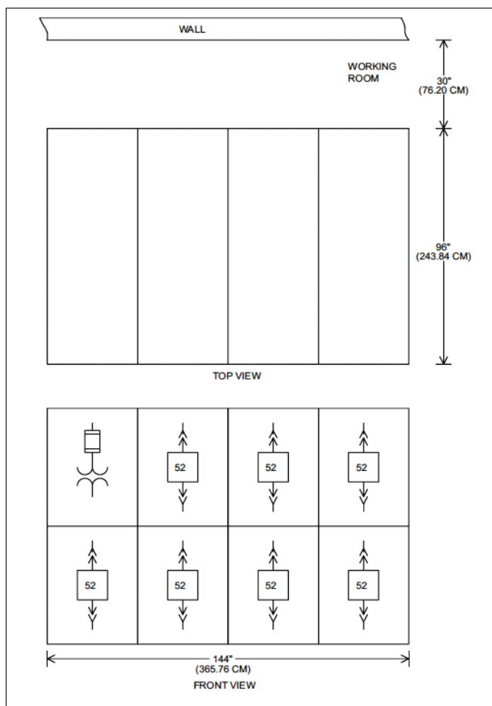
Figure 5. Standard metal-clad switchgear
