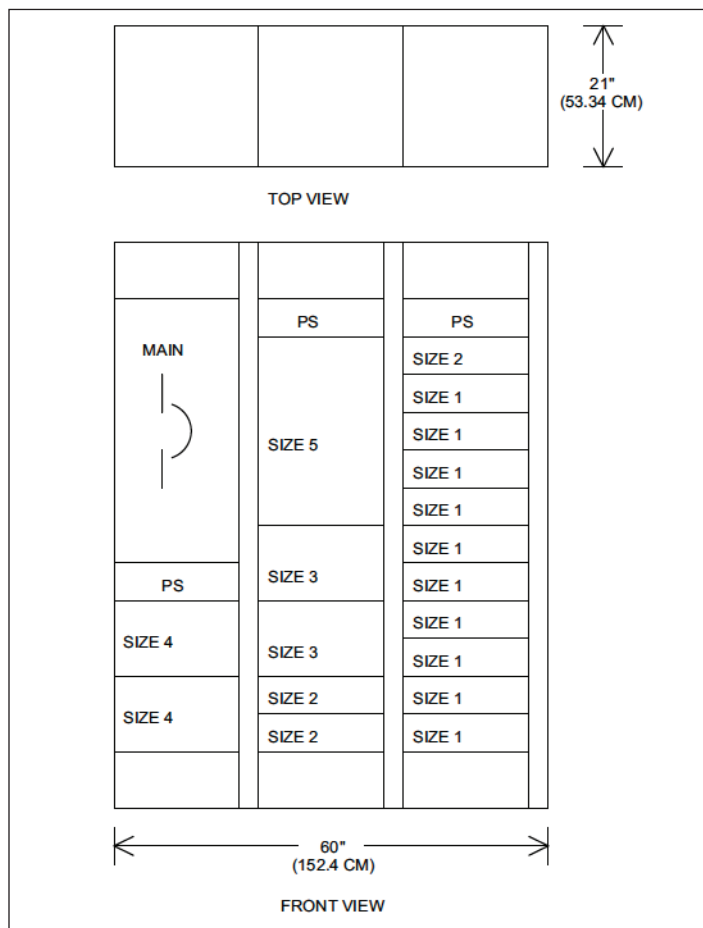
Figure 4. Advanced design IT MCC (IT MCC)
