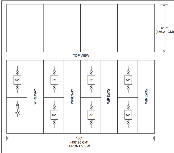
Figure 6. New metal-enclosed vacuum breaker switchgear
