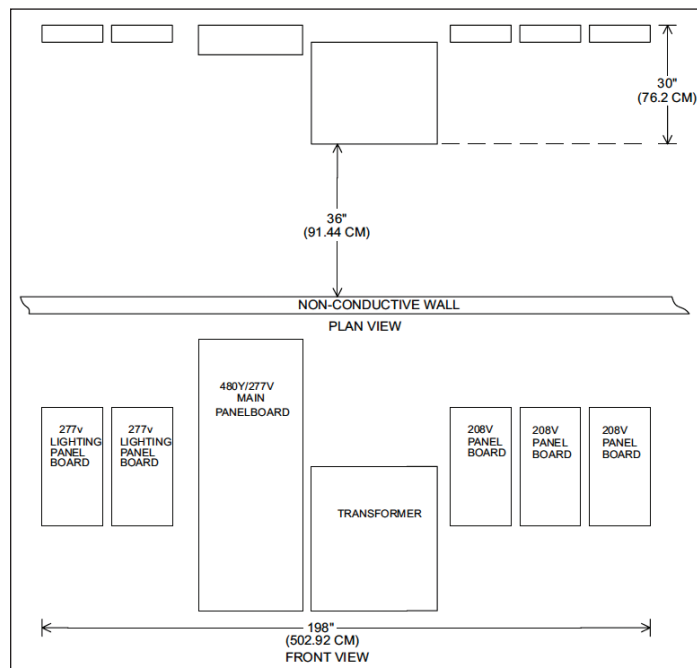
Figure 1. Conventional panelboard/transformer room layout
