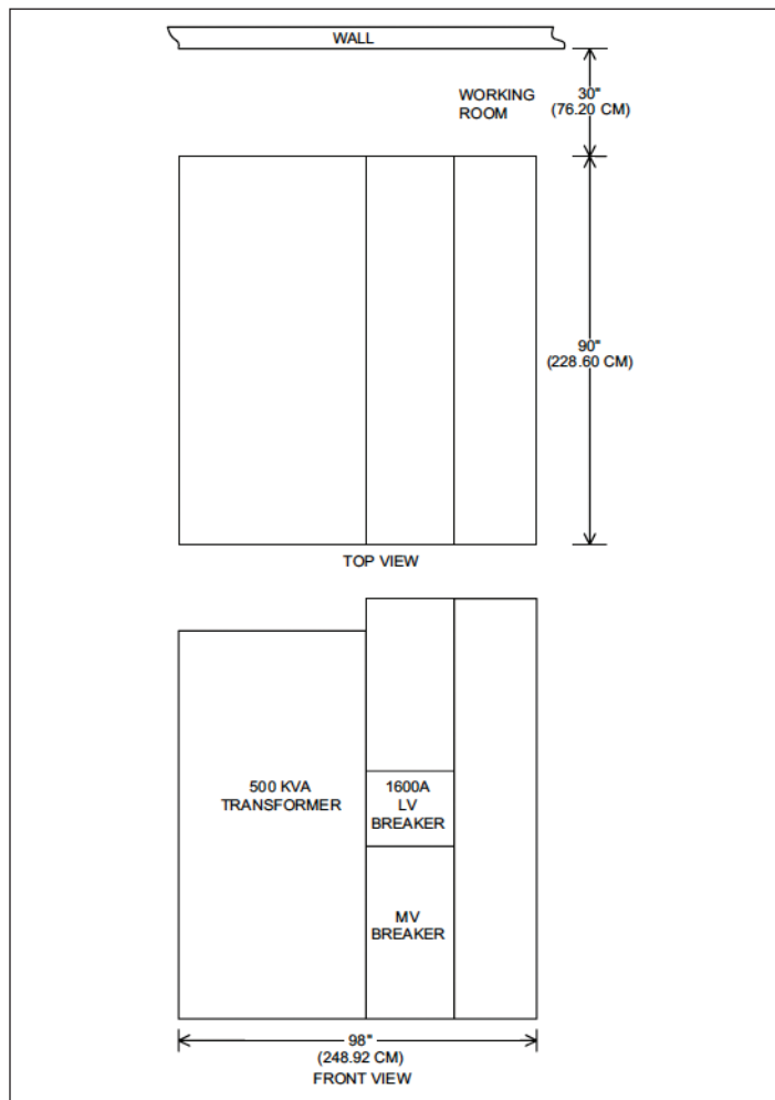
Figure 8. Integrated unit substation (IUS)
