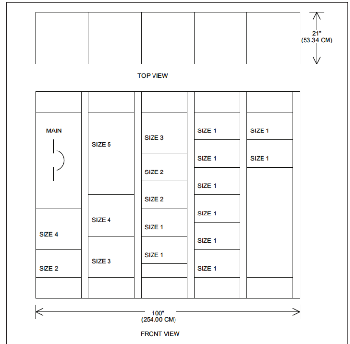
Figure 3. Conventional motor control center (MCC)
