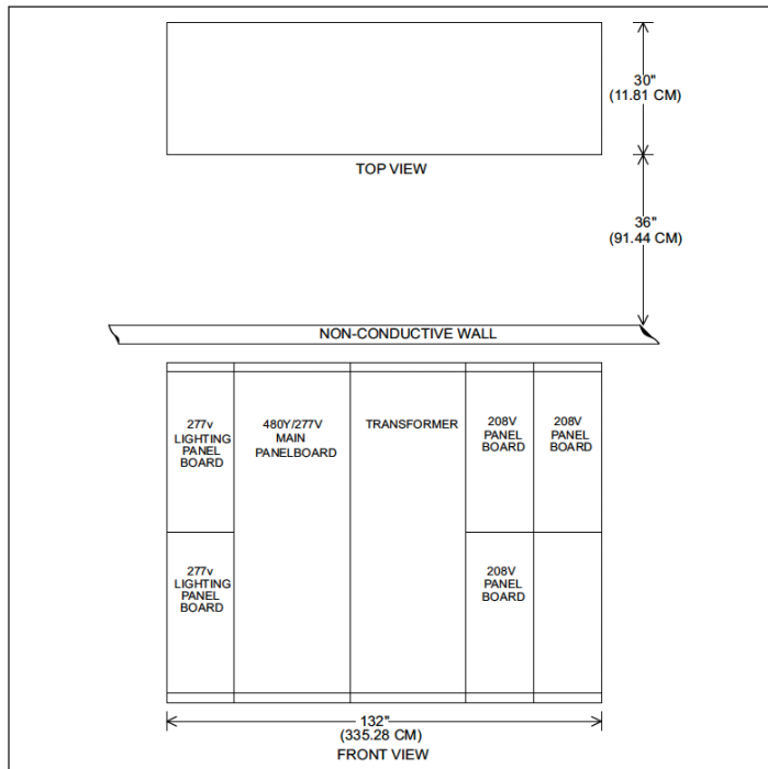
Figure 2. Integrated Facilities Switchboard (IFS)
