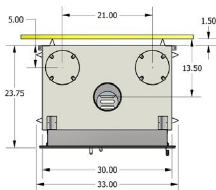
Figure 11 – Parallel Installation
