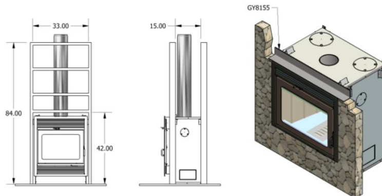
Figure 16 – Framing
