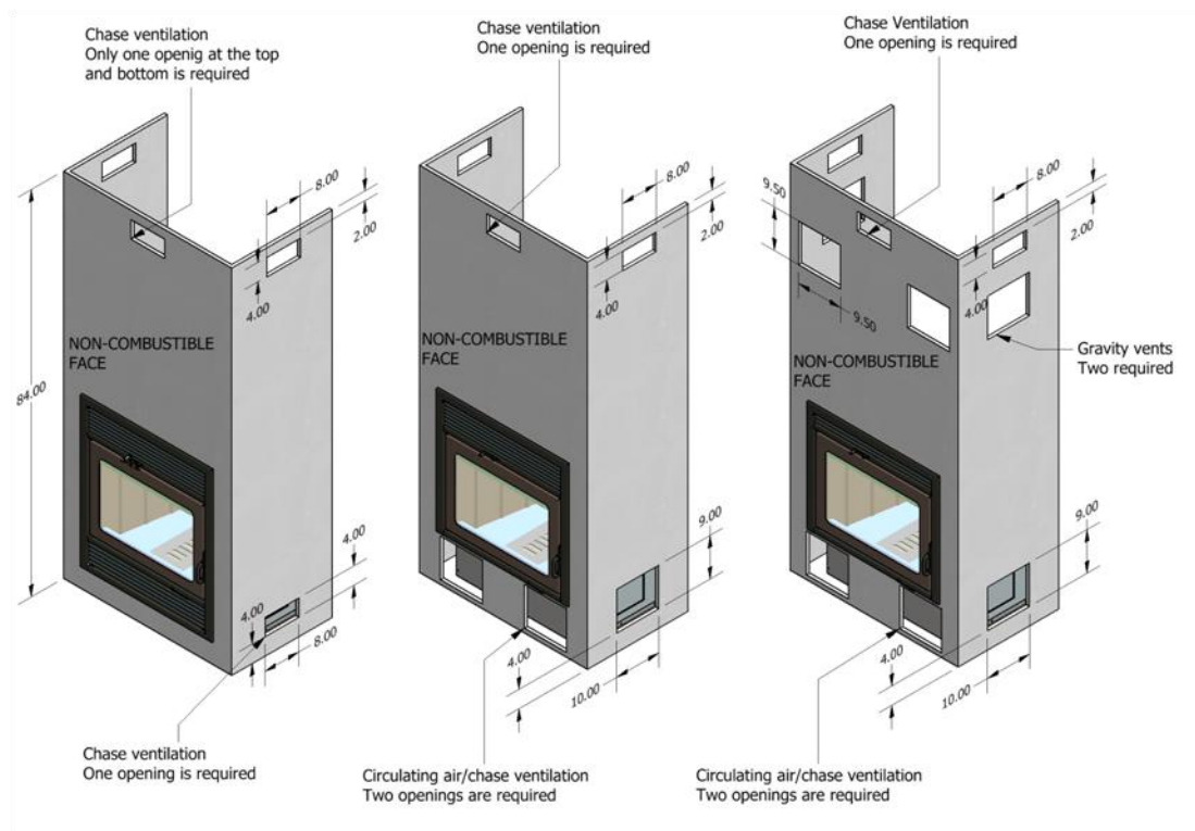
Figure 20 – Chase Ventilation
