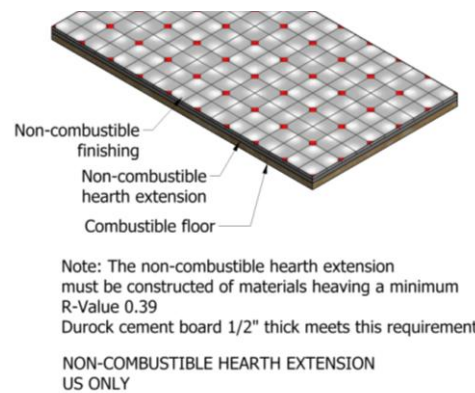
Figure 19 – Non-Combustible Hearth Extension. U.S. Installations Only
