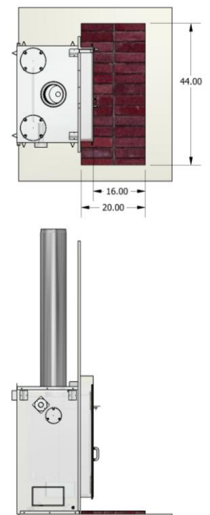
Figure 18 – Hearth Extension
