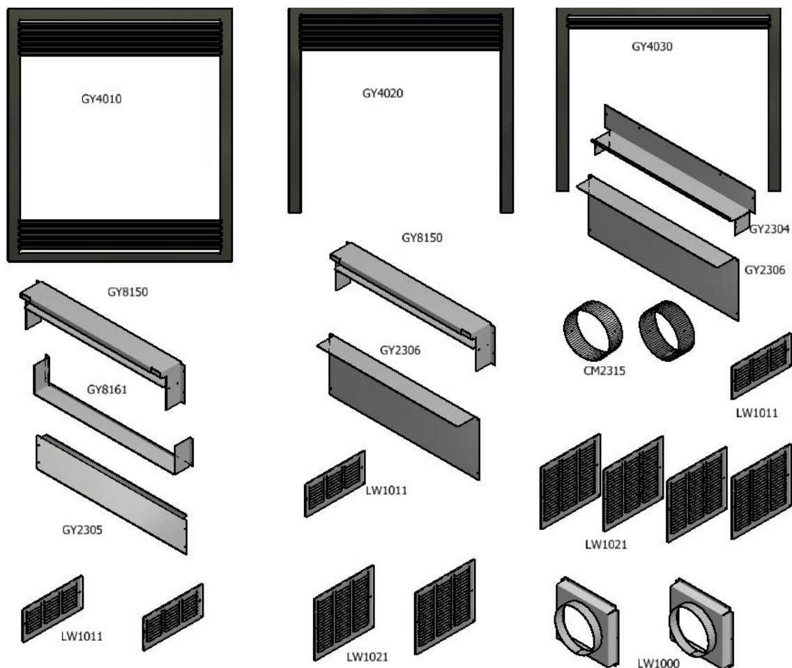
Figure 14 – Classic, Semi-Classic and Clean Face Parts Required
