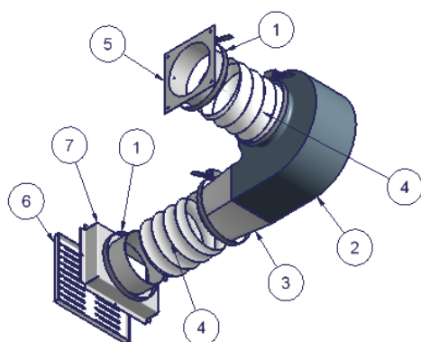
Figure 30 – Hot Air System
