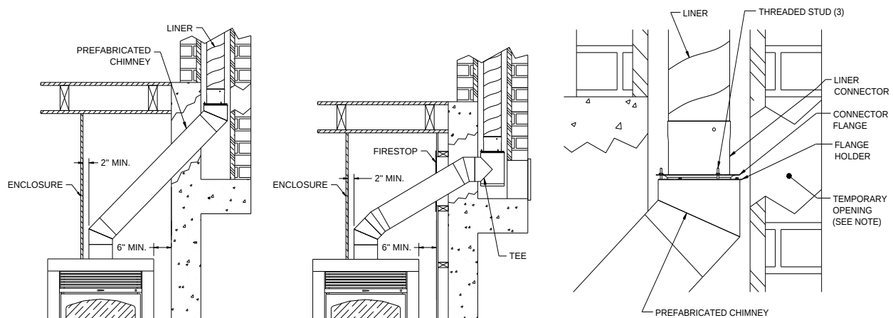
Figure 27 – Connection to a Masonry Chimney
