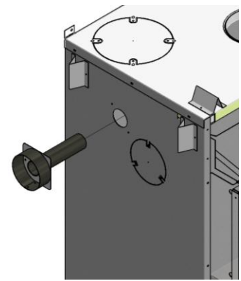
Figure 28 – Fresh Air Adaptor
