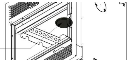
Figure 6 – The Chimney Sweeping Cap
