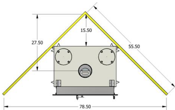
Figure 12 – Corner Installation
