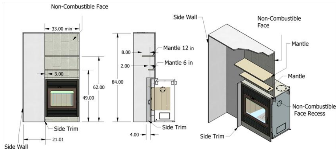
Figure 21 – Clearances to Combustibles
