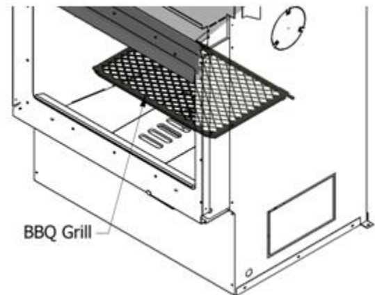
Figure 5 – Barbecue Grill
