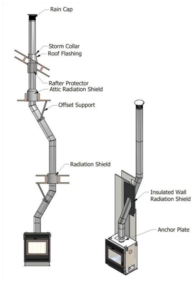
Figure 25 – Chimney Installation
