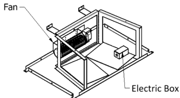
Figure 22 – Fan Kit
