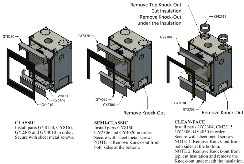
Figure 13 – Classic, Semi-Classic and Clean Face Installations
