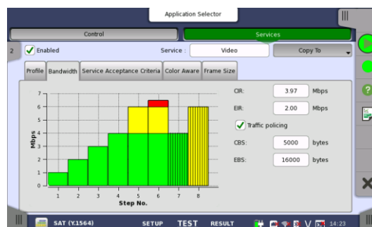
Fig. 7. Bandwidth Settings
