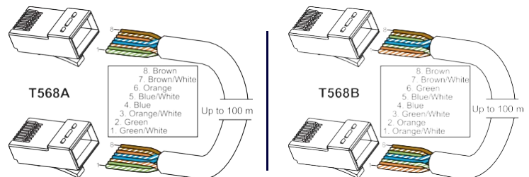
FIG. 4 RJ-45 PINOUTS
