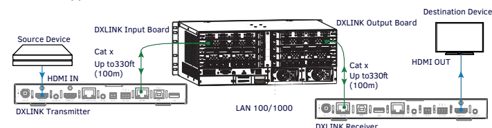
FIG. 2 DXLINK TX AND RX AS ENDPOINTS WITH COMPATIBLE DXLINK EQUIPMENT
