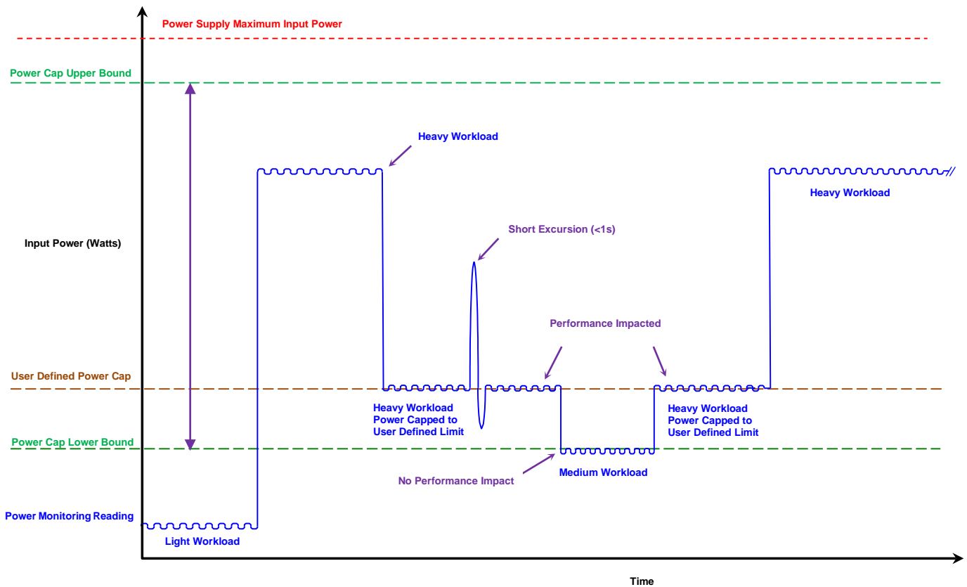
Figure 20 Power capping example
