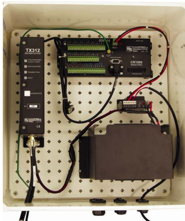
FIGURE 3-3. DCP Enclosure
