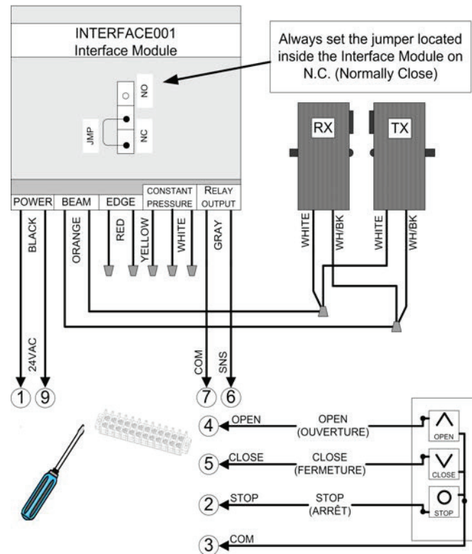
Figure 2 - PHOTO008A/B/C/D - Connection to Electromechanical Operator Without 3-PBS Constant Pressure-to-Close Revert Mode
